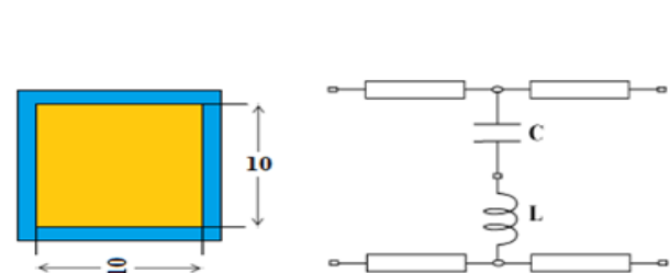
Fig. 7. Geometry of an AMC unit cell with its typical equivalent circuit.
