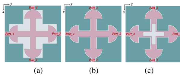
Fig. 2. Antenna design process. (a) Ant1. (b) Ant2. (c) Ant3.
