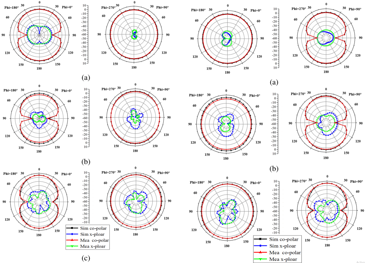
Fig. 8. Simulated and measured radiation patterns in vertical. (a) xoz and yoz plane at 2.3 GHz. (b) xoz and yoz plane at 4.0 GHz. (c) xoz and yoz plane at 5.4 GHz.
