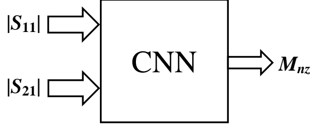
Fig. 2. The circuit model-based CNN for coupling matrix extraction.
