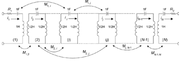
Fig. 1. Equivalent circuit of an N -coupled resonator filter [24].
