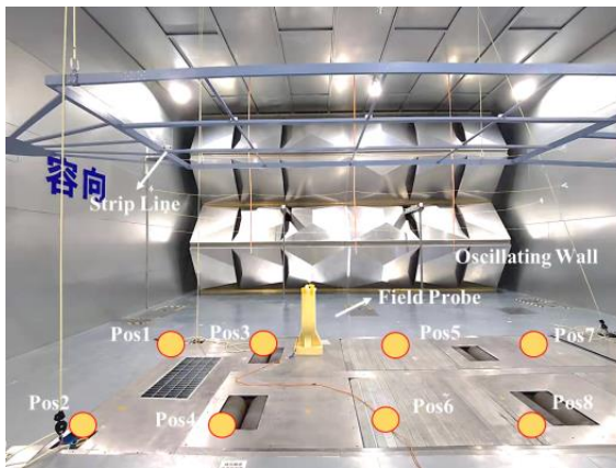
Fig. 6. Typical FU measurement setup with the TLS: (a) schematic plot, and (b) measurement scenario in an RC.
