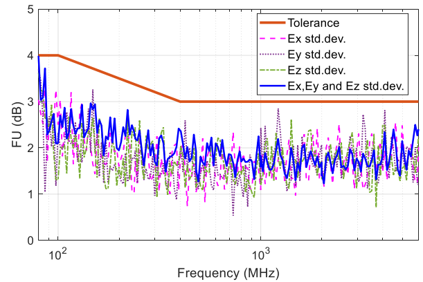
Fig. 10. The FU in the RC using oscillating wall compared with the tolerance requirements from 80 MHz - 6 GHz.
