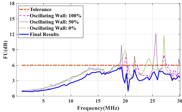
Fig. 8. The FU in the RC with different state of the oscillating wall compared with the tolerance requirements from 0 - 30 MHz.
