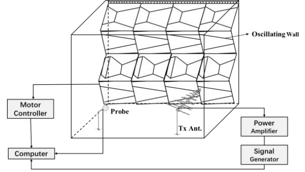
Fig. 9. Typical FU measurement setup using an oscillating wall.
