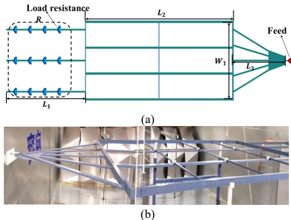
Fig. 1. The designed strip line. (a) Geometry structure. (b) Fabricated sample.
