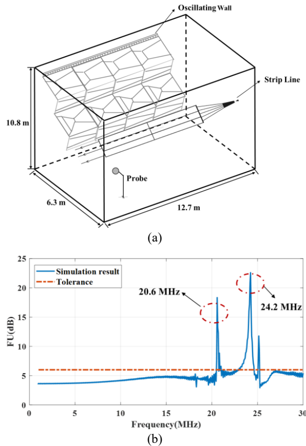
Fig. 2. (a) The initial hybrid system. (b) The simulation results of FU in an RC.
