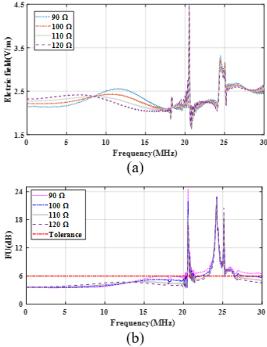
Fig. 3. From 0 to 30 MHz, the simulation results changing with the value of load in an RC, (a) E-field for 1 W input power and (b) FU.
