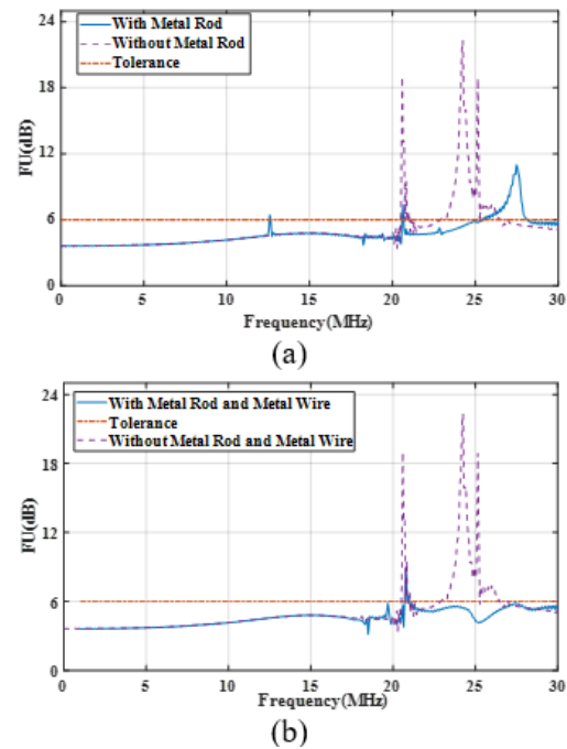
Fig. 5. The optimizing simulation results of FU in an RC compared with the tolerance requirements combining (a) metal rod, and (b) metal rod and metal wire.
