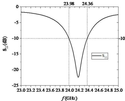
Fig. 6. The simulated reflection coefficients of the series-fed five-element patch linear array.
