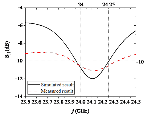
Fig. 8. The simulated and measured reflection coefficients of the planar array antenna.
