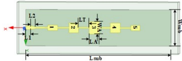
Fig. 1. The structure of the series-fed five-element patch linear array.
