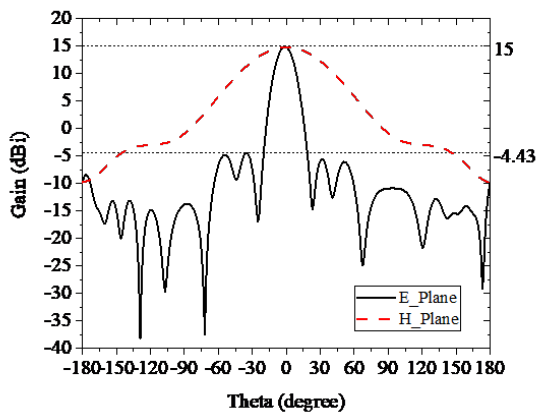
Fig. 7. The simulated radiation patterns of the series-fed five-element patch linear array.
