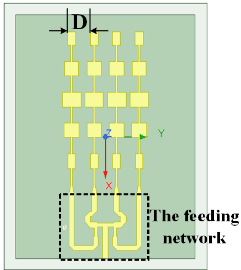
Fig. 2. The structure of the 5×4 planar array antenna.
