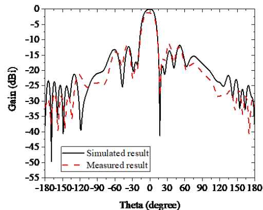
Fig. 9. The simulated and measured E-plane of the planar array antenna.
