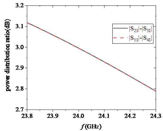
Fig. 4. The simulated power distribution ratio of the feeding network.
