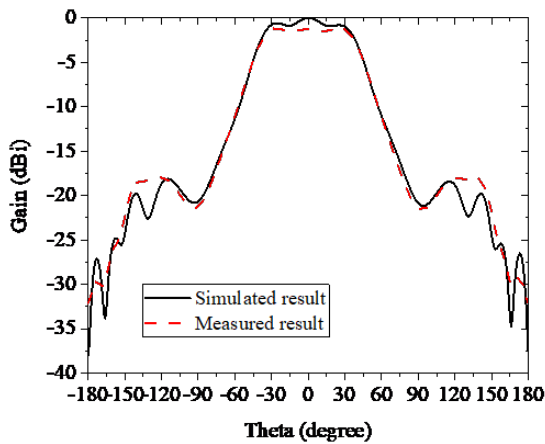
Fig. 10. The simulated and measured H-plane of the planar array antenna.
