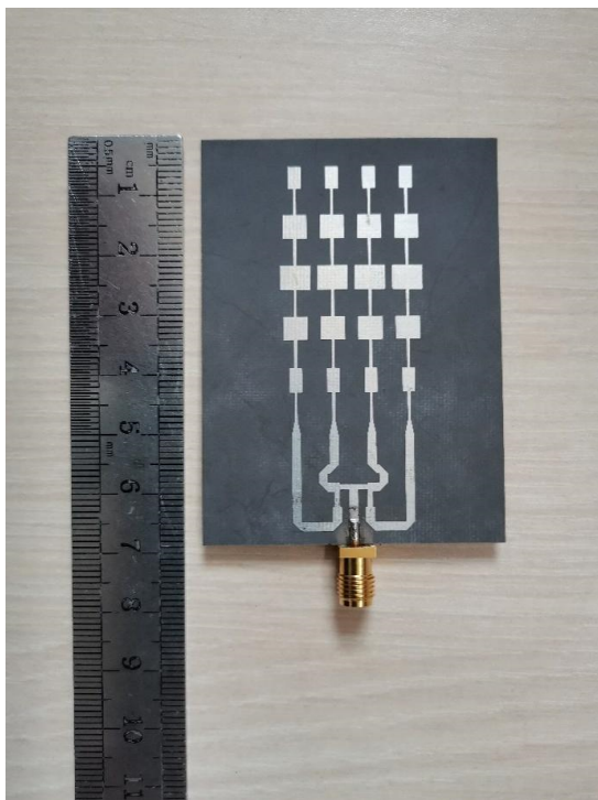
Fig. 3. The fabricated planar array antenna photograph.
