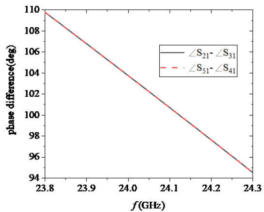
Fig. 5. The simulated phase difference of the feeding network.
