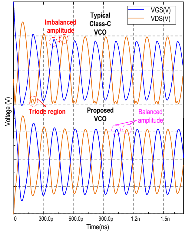
Fig. 8. Simulated drain output voltage.
