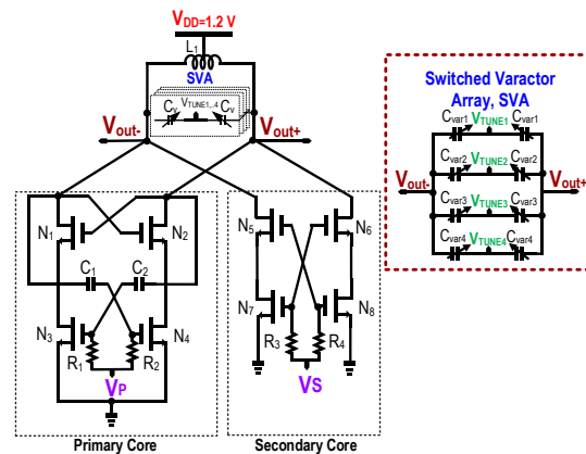
Fig. 2. Proposed LC-VCO with dual core VCO.
