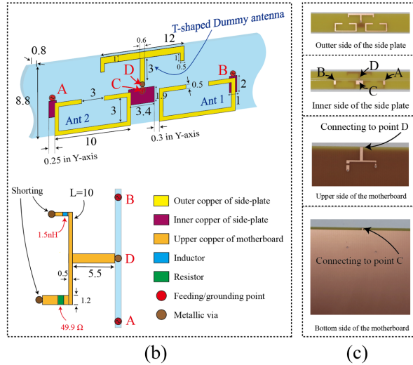
Fig. 2. (a) Configuration of the proposed 4 \times 4 MIMO antenna, (b) zoom-in view of the proposed antenna pair and (c) photos of the fabricated substrate.
