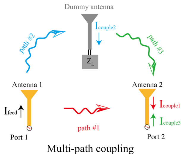
Fig. 1. Decoupling diagram by using dummy antenna.
