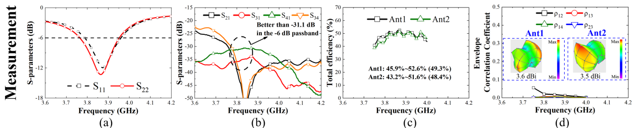
Fig. 6. Measured results of (a) reflection coefficients, (b) transmission coefficients, (c) total efficiencies, and (d) envelope correlation coefficient.
