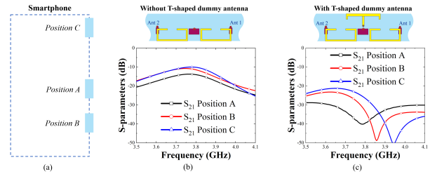
Fig. 4. S-parameter of proposed antenna pair located in different places, (a) antenna placing diagram, (b) S-parameters of the antenna pair without T-shaped dummy antenna and (c) S-parameters of antenna pair with T-shaped dummy antenna.
