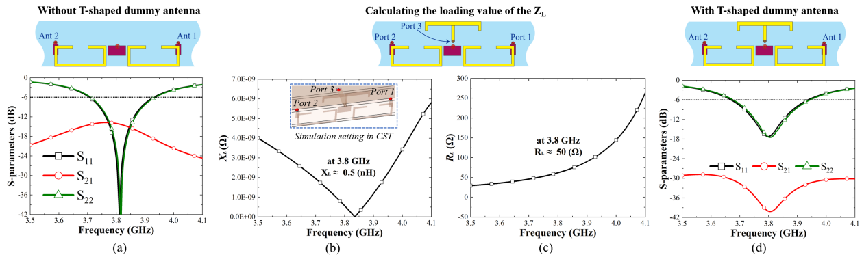
Fig. 3. (a) Simulated results of antenna pair without T-shaped dummy antenna; (b) and (c) is the simulated loading requirement of the T-shaped dummy antenna, and (d) is the simulated result of antenna pair with T-shaped dummy antenna.
