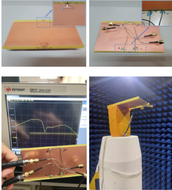
Fig. 7. Fabricated prototype and measurement setup.
