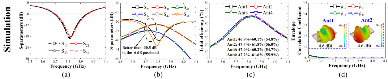
Fig. 5. Simulated results of (a) reflection coefficients, (b) transmission coefficients, (c) total efficiencies, and (d) envelope correlation coefficient.
