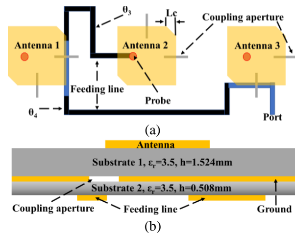
Fig. 1. Geometries of the proposed CP patch antennas decoupling method. (a) Top view. (b) Lateral view. ( L_c=2.4\text{mm} , \theta_3=470^\circ and \theta_4=860^\circ .)
