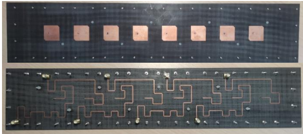
Fig. 4. Photograph of the fabricated 1 \times 8 antenna array.
