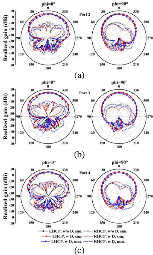
Fig. 8. Measured and simulated radiation patterns of representative ports. (a) Port 2. (b) Port 3. (c) Port 4.
