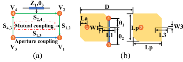
Fig. 2. Configuration of the decoupling between Antennas 1 and 2. (a) Signal flow diagram. (b) Simplified four-port model. ( \theta_1=45^\circ , \theta_2=90^\circ , and L_a = 6.8 mm, L_1=4.6 mm, L_3=4 mm, W_1=W_3=0.2 mm, L_p=22.7 mm.)
