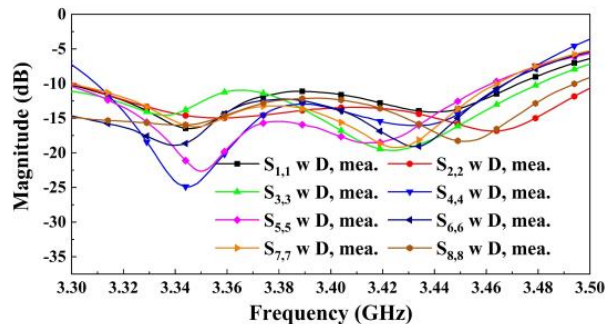
Fig. 5. Measured scattering parameters of the fabricated 1 \times 8 array.
