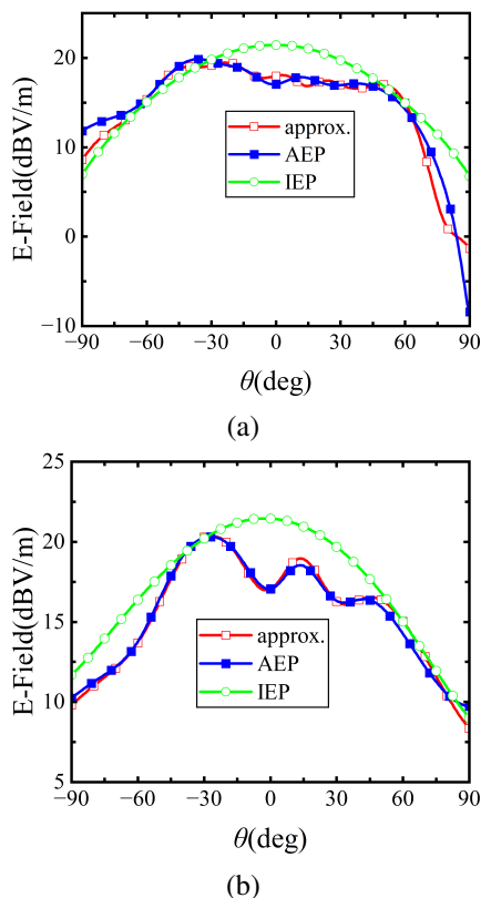
Fig. 2. The compensated pattern of 29-th element (a) xoz -plane, (b) yoz -plane.
