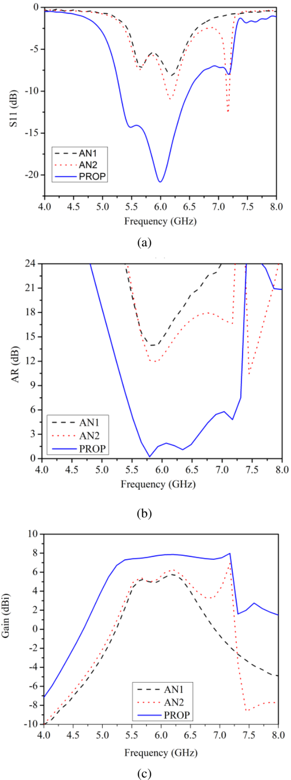
Fig. 5. Simulated results of three antenna versions in (a) S_{11} , (b) AR, and (c) gain.
