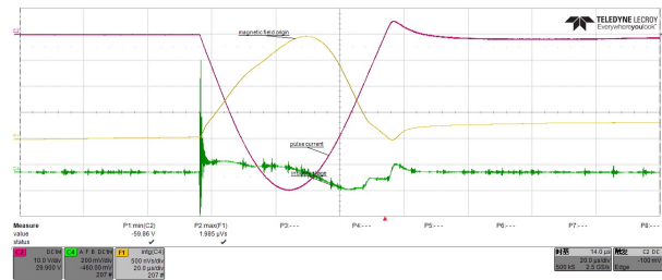
Fig. 13. Induced voltage and integration of leakage field.
