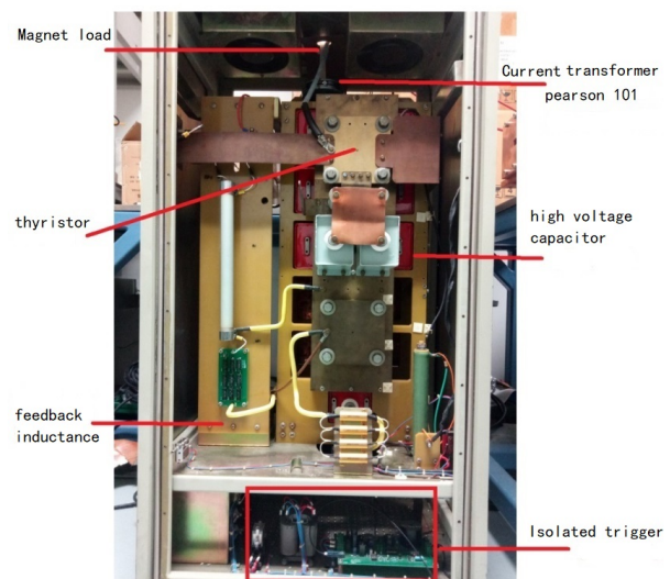
Fig. 8. Layout of excitation pulse power supply.
