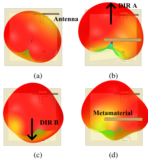
Fig. 16. Measured 3D radiation patterns: (a) no MTM in 2450 MHz MTM, (b) with MTM in 2450 MHz, (c) no MTM in 5400 MHz, and (d) with MTM in 5400 MHz.
