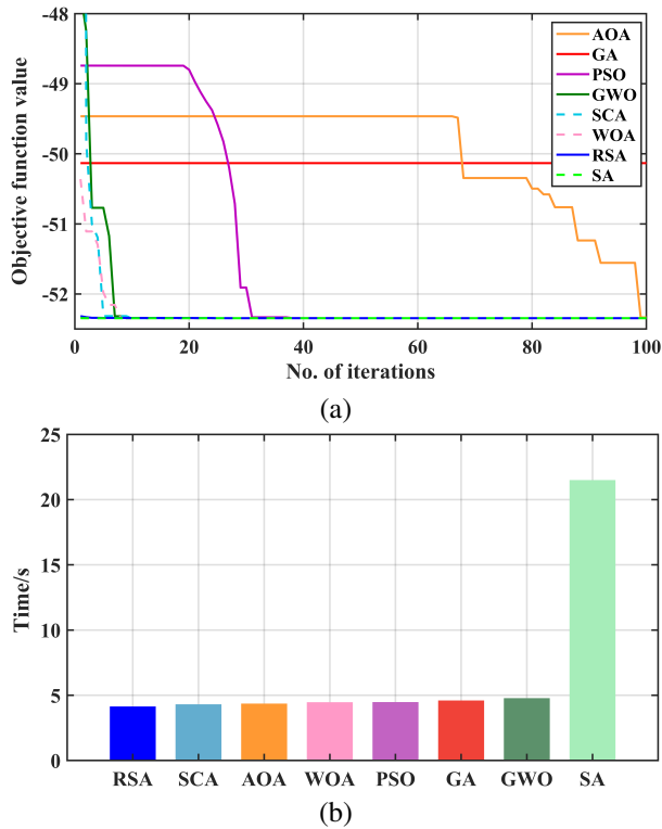
Fig. 5. (a) Convergence results of maximum likelihood estimation and (b) computation time of each algorithm.
