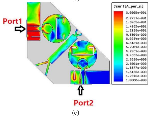
Fig. 9. Simulated surface current distribution when Port 1 acts as the exciter: (a) 3.4 GHz, (b) 5.25 GHz, and (c) 7.5 GHz.
