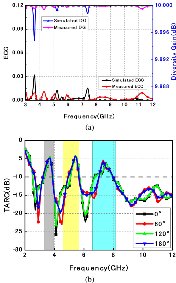
Fig. 13. Simulated or measured results. (a)ECC and DG. (b) TARC.
