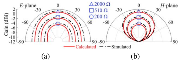
Fig. 6. Calculated and simulated gain patterns at 5.8 GHz of the infinite-ground model under different loaded resistance: (a) E-plane patterns and (b) H-plane patterns.
