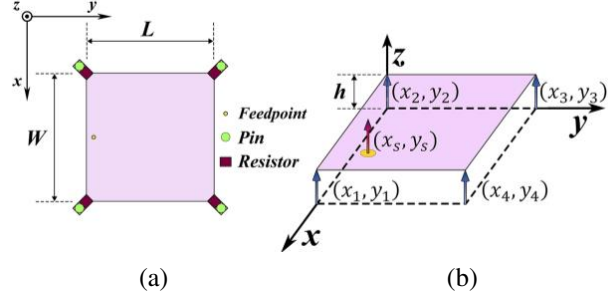
Fig. 2. The proposed resistor-loaded patch antenna and its cavity model: (a) Configuration and (b) equivalent cavity model.
