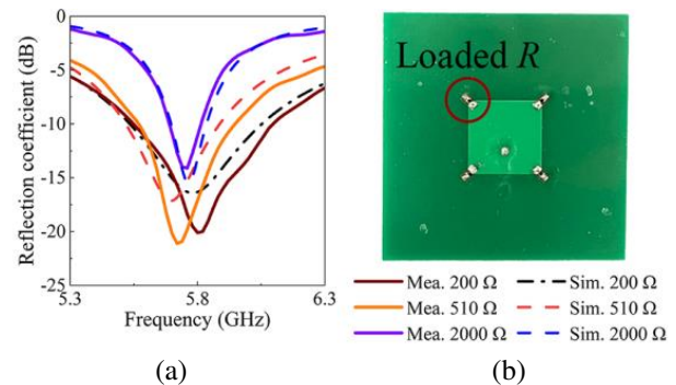
Fig. 8. (a) Simulated and measured reflection coefficient of the fabricated patch antennas; (b) photograph of the fabricated prototype.
