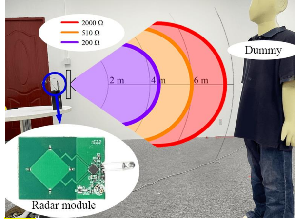
Fig. 11. Photograph of the test site and the fabricated radar module. The measured recognition scopes of indoor motion radar modules loaded with 200- \Omega , 510- \Omega , and 2000- \Omega resistors are also illustrated. (The installation height is 0.9 m).
