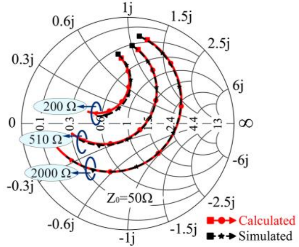
Fig. 4. Calculated and simulated input impedances in the Smith Chart under different loaded resistance within frequency range of 5.3 to 6.3 GHz.
