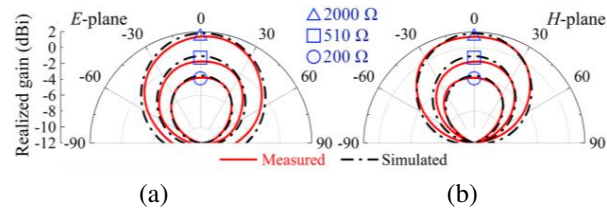
Fig. 10. The radiation patterns of the antenna prototypes at 5.8 GHz: (a) E-plane and (b) H-plane.
