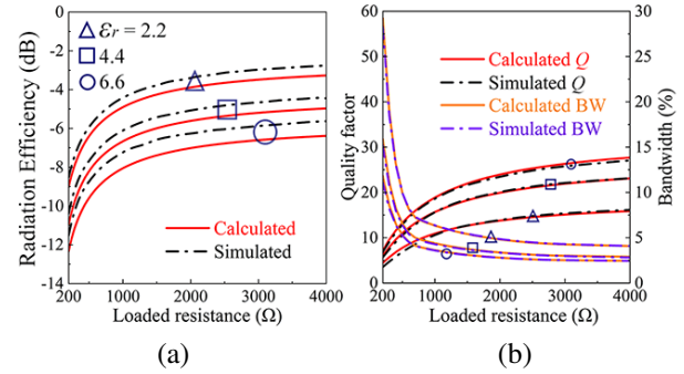
Fig. 7. Calculated and simulated results of (a) radiation efficiency and (b) quality factor and bandwidth for 10-dB return loss. The substrate thickness is 0.8 mm.
