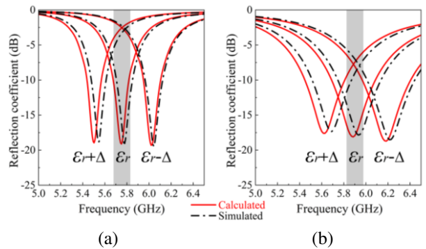
Fig. 5. Calculated and simulated reflection coefficients of the resistor-loaded patch antenna under different relative dielectric permittivity ( \epsilon_r = 4.4 , \Delta = 0.4 ): (a) Patch antenna without resistors and (b) patch antenna with 510 \Omega resistors loaded.
