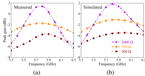
Fig. 9. Peak gain of the antenna prototypes in the frequency range of 5.3 to 6.3 GHz: (a) Measured results and (b) simulated results.
