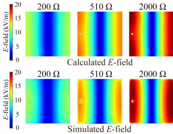
Fig. 3. Calculated and simulated E -field magnitude distributions of resistor-loaded patch antenna loaded with 200 \Omega , 510 \Omega , and 2000 \Omega resistors. The feeding powers are fixed to 1 W.
