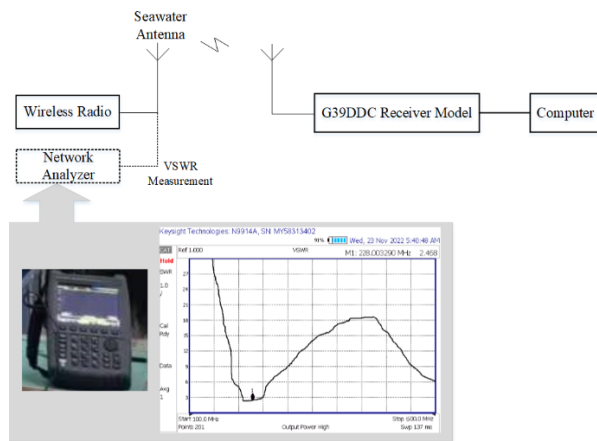
Fig. 7. Experiment of the transceiver system.
