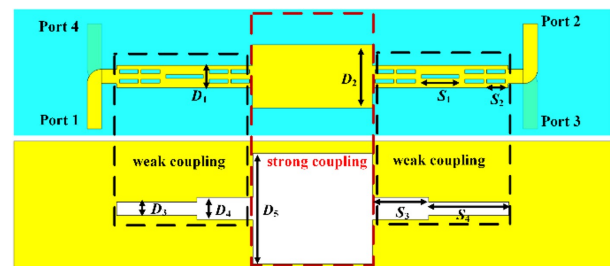
Fig. 5. Top view of the three-section coupled-line coupler.
