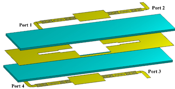
Fig. 4. 3D schematic of the three-section coupled-line coupler.
