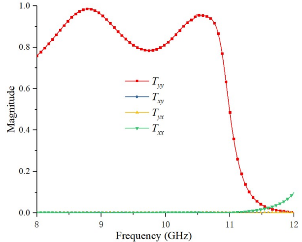
Fig. 2. Transmission coefficients of the proposed metasurface unit cell with s = 0.1 mm.
