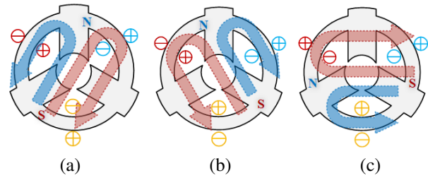
Fig. 4. Armature reaction field of ETW-HSPMSM: (a) time 2, (b) time 3, and (c) time 4.
