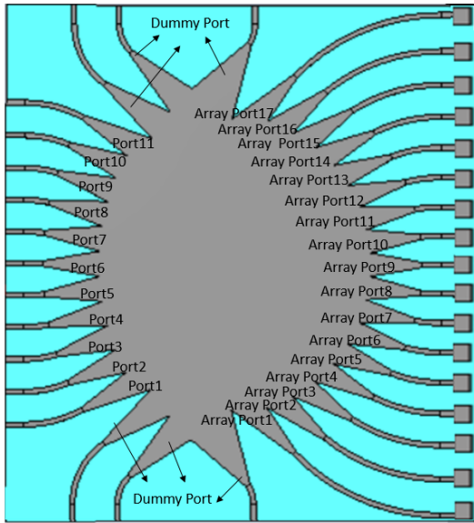
Fig. 5. CST implementation of the lens design.
