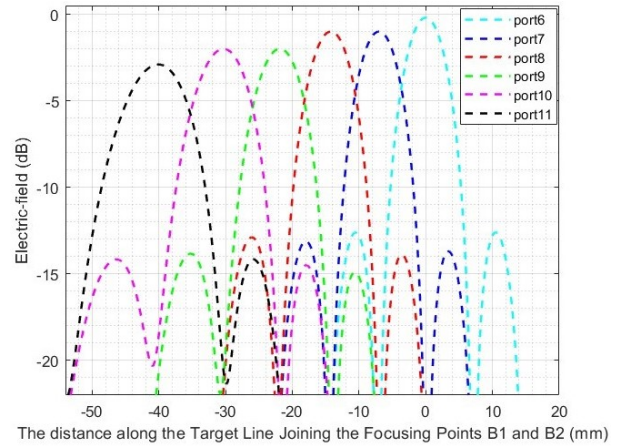
Fig. 6. Radiation patterns for the lens design in Fig. 2 ( g=1.25 ) using CST method.
