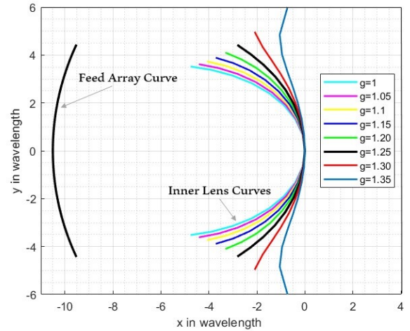
Fig. 2. Lens curves for g=1, 1.05, \dots, 1.35 .
