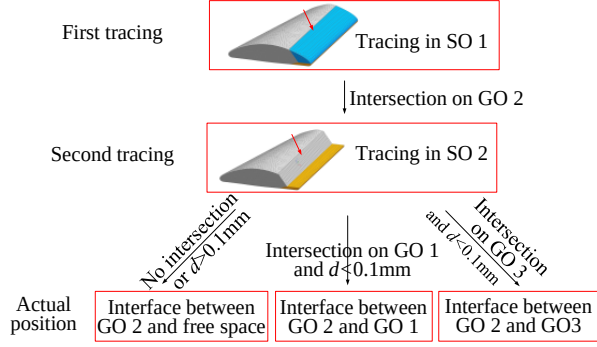
Fig. 8. Ray tracing in multiple scenes.
