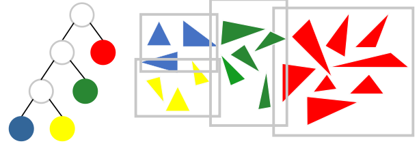
Fig. 3. BVH structure.
