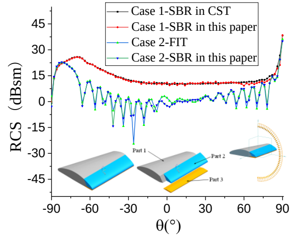
Fig. 13. RCS of three-part combination.
