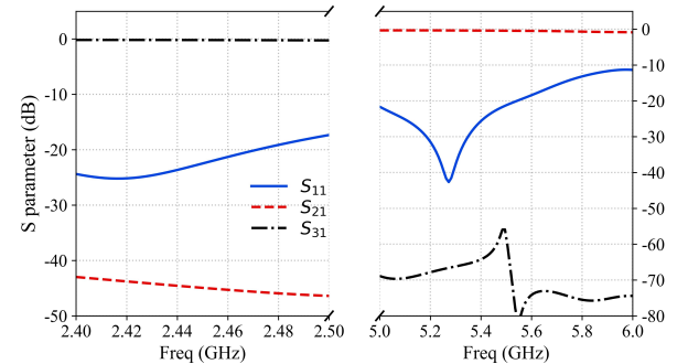
Fig. 11. Simulated S-parameters of the duplex filter.
