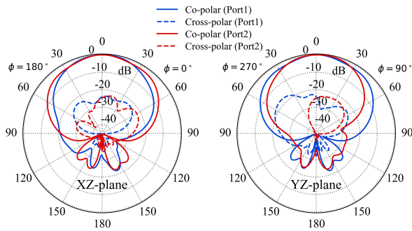
Fig. 7. High-frequency antenna radiation pattern at 5.8 GHz.
