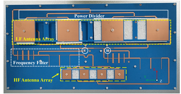
Fig. 8. Prototype of the dual-frequency dual-polarization antenna.
