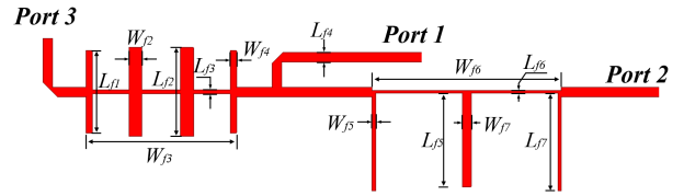
Fig. 10. Geometry of the duplex filter.
