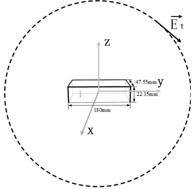
Fig. 4. Waveguide antenna and enclosing sphere.
