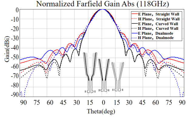
Fig. 6. 118 GHz far-field pattern.
