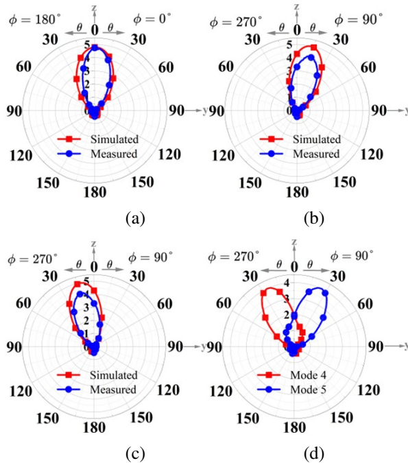
Fig. 11. Measured and simulated radiation patterns for different modes of yoz: (a) Mode 1, (b) Mode 2, (c) Mode 3, and (d) Modes 4 and 5.
