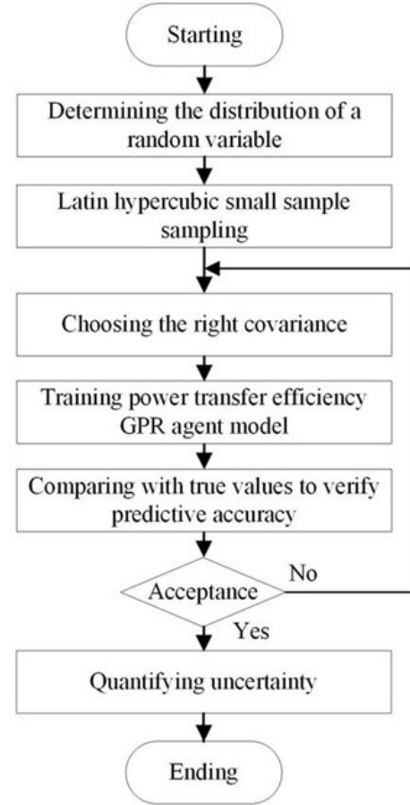
Fig. 4. UQ flow chart of EV-WPT system transmission efficiency.
