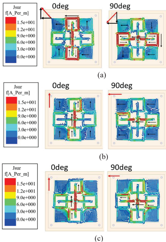
Fig. 6. Simulated current distributions of the antenna. (a) 1.45 GHz, (b) 1.8 GHz, and (c) 2.4 GHz.
