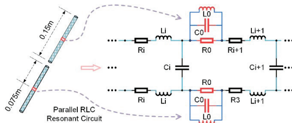
Fig. 14. A dipole loaded with parallel RLC circuit.
