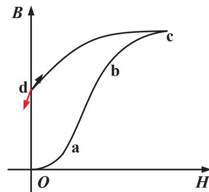
Fig. 2. Hysteresis curve of magnetic material in the transformer core.
