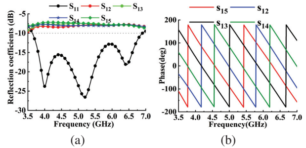
Fig. 6. Simulated results of the broadband feeding network: (a) Reflection coefficient, (b) phase shift.
