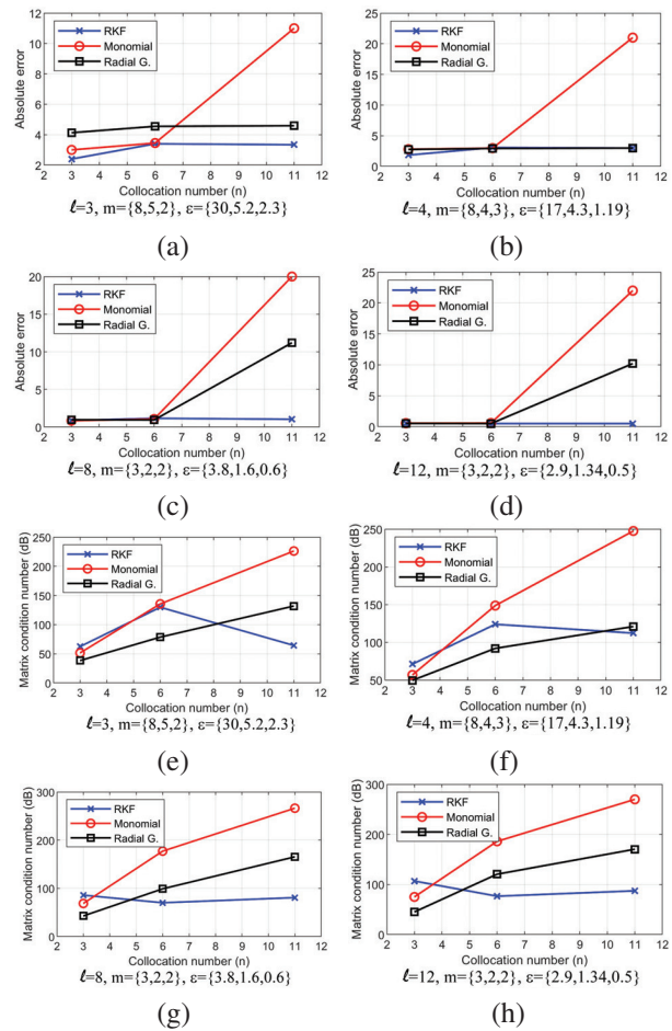
Fig. 6. Error and stability analysis results at \ell = \{3, 4, 8, 12\} . m and \epsilon values are given with respect to the collocation numbers n = \{3, 6, 11\} .
