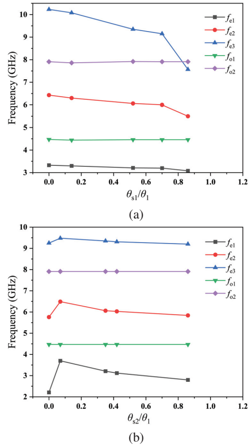
Fig. 4. (a) Even- and odd-mode frequencies ( f_{e1}, f_{e2}, f_{e3}, f_{o1}, f_{o2} ) under variation of \theta_{s1} ; (b) even- and odd-mode frequencies ( f_{e1}, f_{e2}, f_{e3}, f_{o1}, f_{o2} ) under variation of \theta_{s2} .
