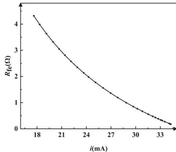
Fig. 9. Variation of equivalent resistance with the current.
