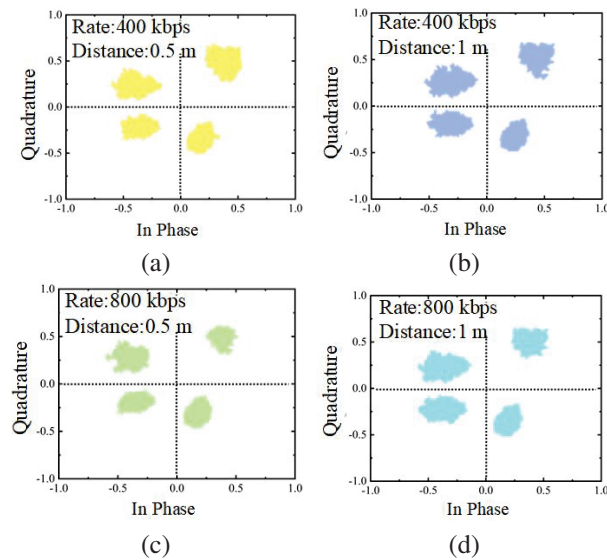
Fig. 7. Relationship between communication performance, transmission rate, and transmission distance. (a) Data rate: 400 kbps, distance: 0.5 m, (b) data rate: 400 kbps, distance: 1 m, (c) data rate: 800 kbps, distance: 0.5 m, and (d) data rate: 800 kbps, distance: 1 m.
