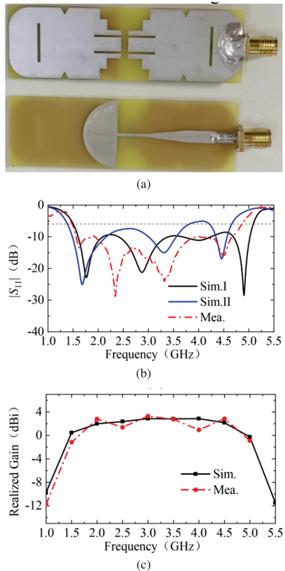
Fig. 4. Fabricated 10:1 scaled antenna element and its experiment results: (a) top view and bottom view, (b) simulated and measured |S_{11}| , and (c) simulated and measured gain.
