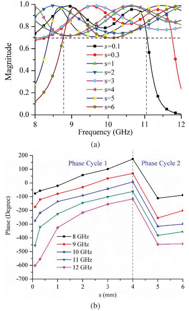
Fig. 4. (a) Transmission magnitude of unit cell. (b) Transmission phase of unit cell.
