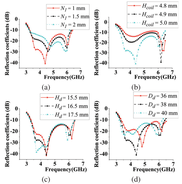
Fig. 6. Reflection coefficients versus antenna parameters: (a) length of joint N_1 , (b) coil height H_{coil} , (c) dielectric height H_d , and (d) dielectric diameter D_d .
