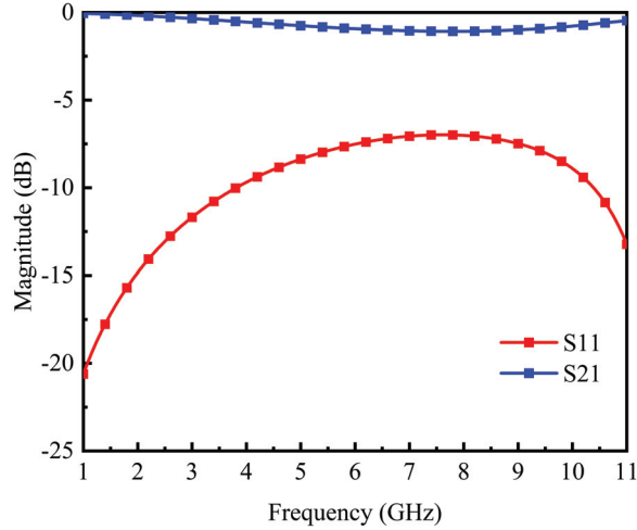
Fig. 7. Simulated S-parameters of the metasurface unit cell.
