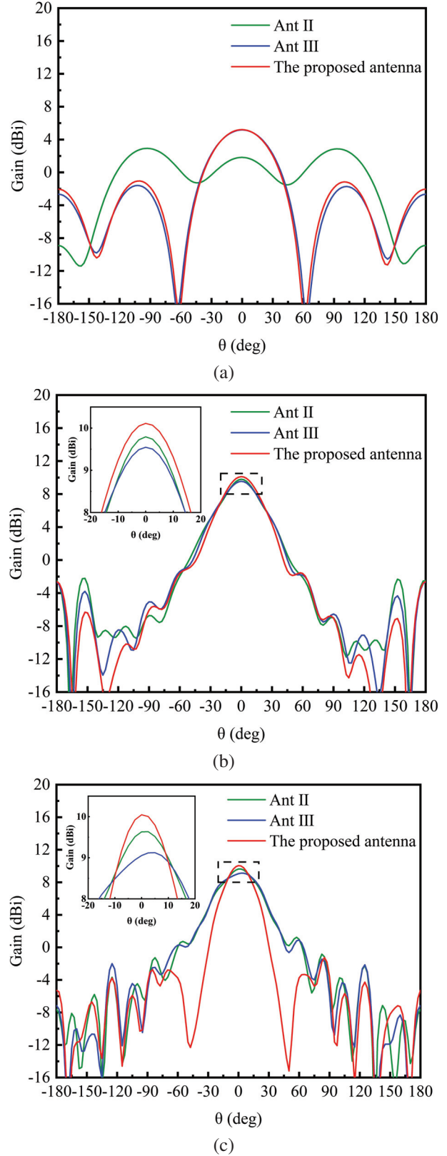
Fig. 4. The far-field radiation pattern in yoz -plane of reference antennas and the proposed antenna at (a) 1.4 GHz, (b) 6 GHz, and (c) 8 GHz.
