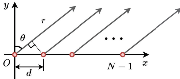
Fig. 1. Schematic diagram of linear array radiation.
