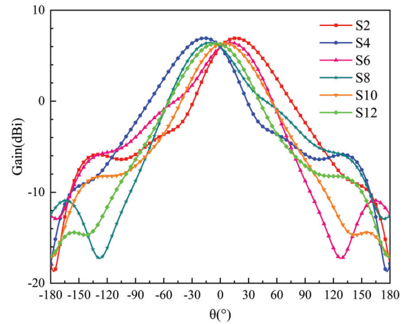
Fig. 9. Simulated radiation pattern in yo z plane at 5 GHz.
