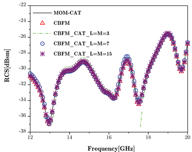
Fig. 5. Wideband BCS of conical radome computed by CBFM-CAT using three different orders.
