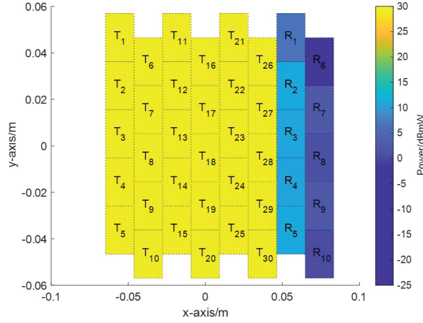
Fig. 2. Distribution characteristics of the coupling self-interference power for simultaneous transmission and reception with the separate sub-apertures array antenna.
