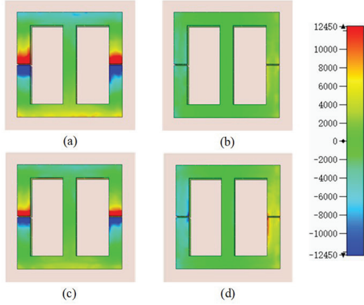
Fig. 3. Electric field distribution of the proposed metasurface unit with s = 0.1 mm: (a) y-polarization incident wave at 9 GHz, (b) x-polarization incident wave at 9 GHz, (c) y-polarization incident wave at 10.5 GHz, and (d) x-polarization incident wave at 10.5 GHz.
