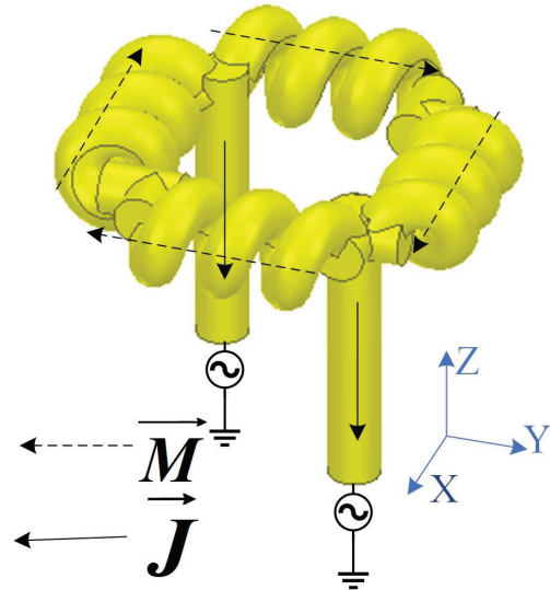
Fig. 3. Equivalent magnetic-current loop and monopole of a coil feeding structure.
