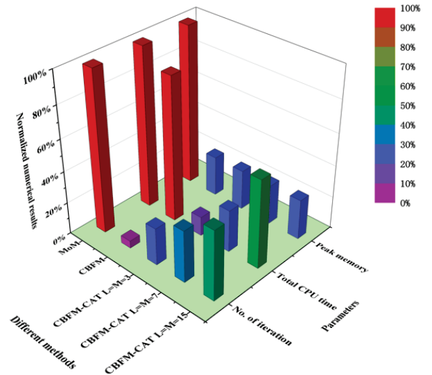
Fig. 9. Comparison of peak memory, CPU time and number of iterations for pyramid radome.
