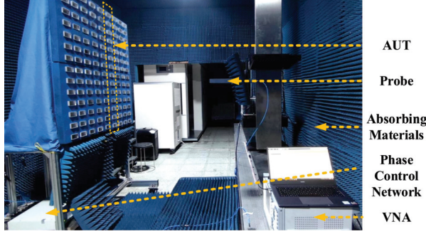
Fig. 3. Measurement environment.
