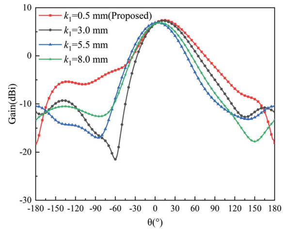
Fig. 10. Simulated radiation pattern in the xoz plane at State 1 varying with k_1 .
