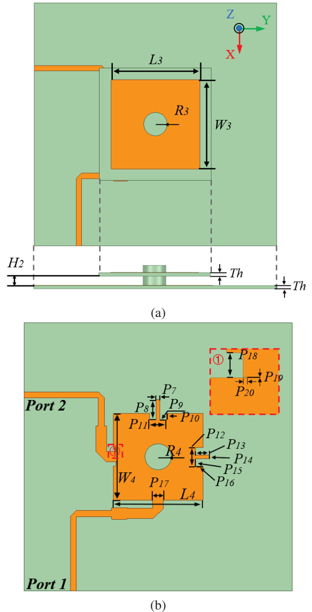
Fig. 5. High-frequency antenna unit: (a) top structure and (b) bottom structure.
