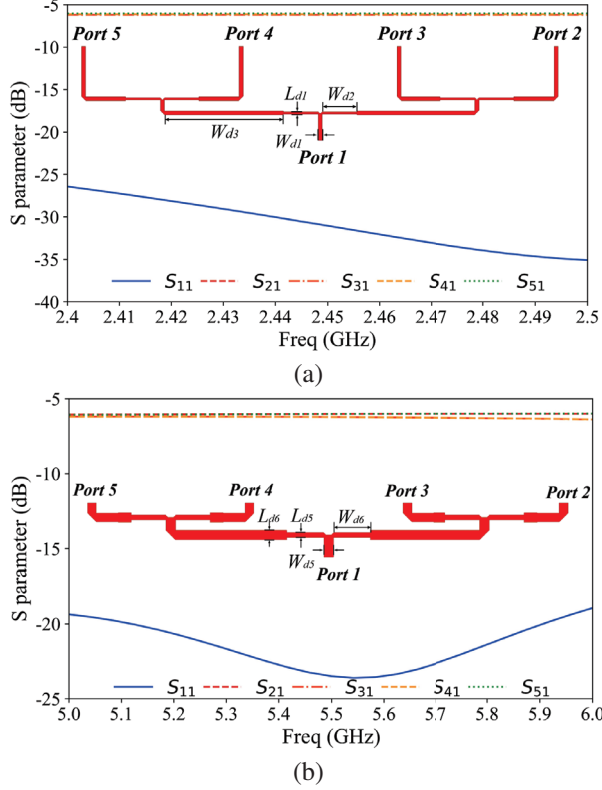
Fig. 9. Simulated S-parameters of power divider: (a) simulated S-parameters of the low-frequency power divider and (b) simulated S-parameters of the high-frequency power divider.
