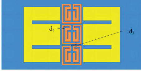
Fig. 6. Front view of the integral MIMO antenna loaded with MTMs. (Blue is the dielectric substrate, the radiation patch is yellow and the MTM structure on the same surface as the radiation patch is orange).
