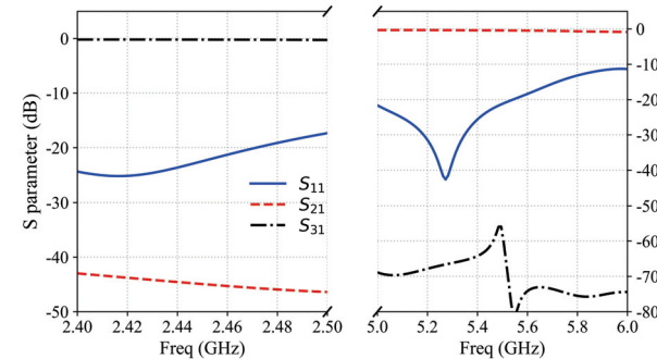
Fig. 11. Simulated S-parameters of the duplex filter.
