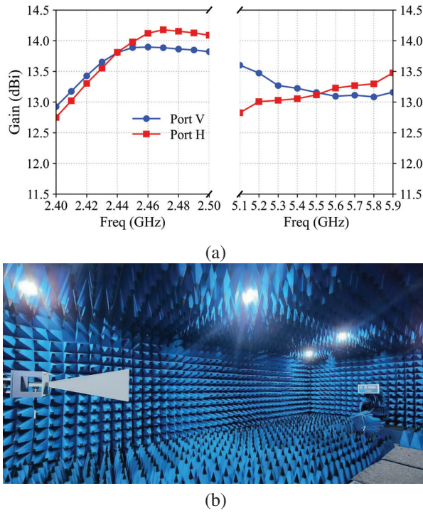
Fig. 15. Measured gains for the proposed antenna: (a) measured gains for port V and port H and (b) antenna measured in chamber.
