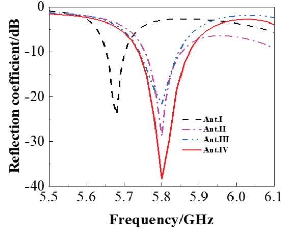
Fig. 4. Simulated reflection coefficient of antennas.
