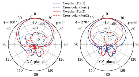
Fig. 7. High-frequency antenna radiation pattern at 5.8 GHz.
