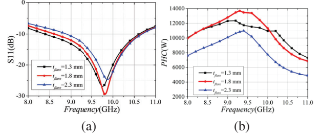
Fig. 4. Simulated results corresponding to different flare thickness values t_{\text{flare}} (a) S11 and (b) PHC.
