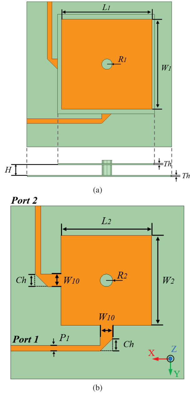
Fig. 2. Low-frequency antenna element: (a) top structure and (b) bottom structure.
