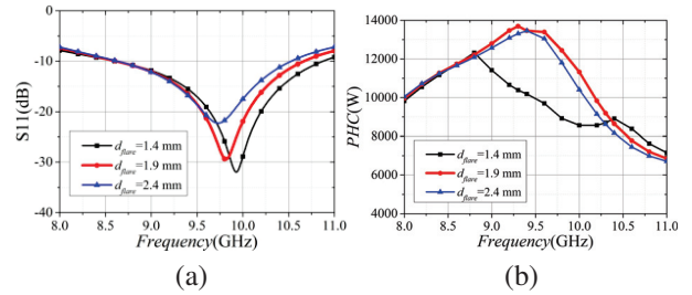
Fig. 6. Simulated results corresponding to different distance values between the two flares d_{\text{flare}} (a) S11 and (b) PHC.
