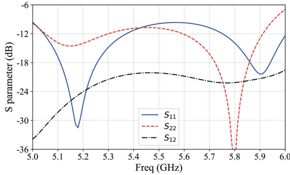
Fig. 6. High-frequency antenna S parameter.
