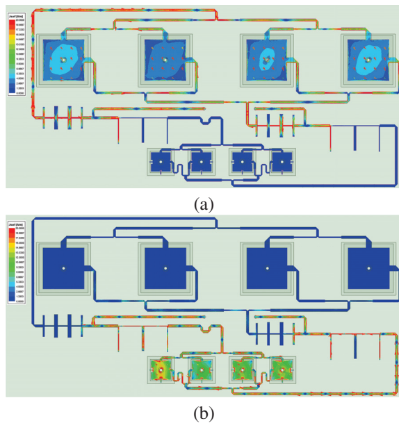
Fig. 12. Current distribution of antenna: (a) currents at 2.45 GHz and (b) currents at 5.8 GHz.
