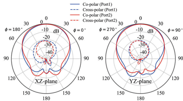
Fig. 4. Low-frequency antenna element radiation pattern at 2.45 GHz.
