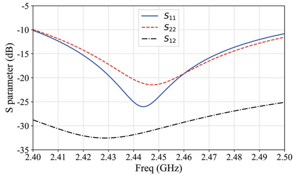
Fig. 3. Low-frequency antenna S-parameter.
