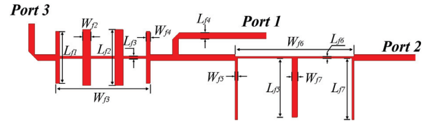
Fig. 10. Geometry of the duplex filter.
