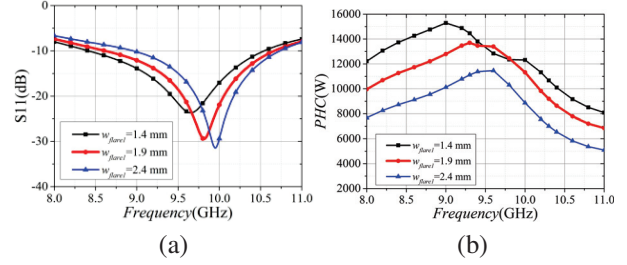
Fig. 5. Simulated results corresponding to different width values of the flare w_{\text{flare1}} (a) S11 and (b) PHC.
