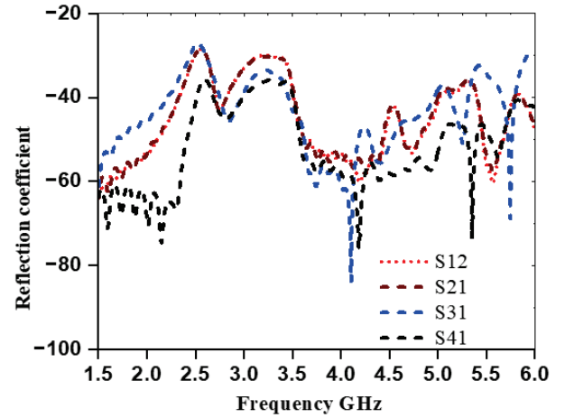
Fig. 6. Transmission coefficients.
