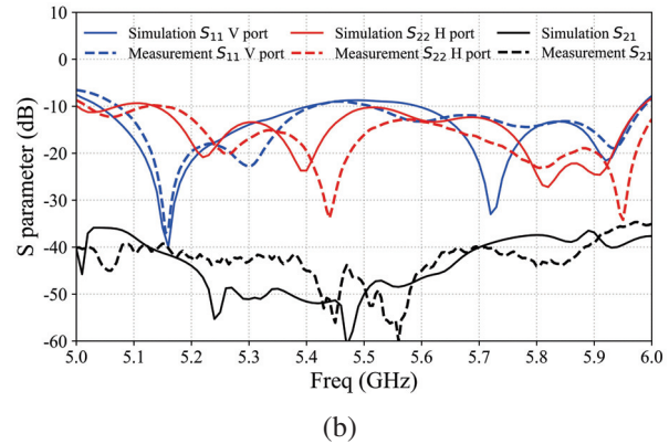
Fig. 13. S-parameters of the proposed antenna: (a) low-frequency band and (b) high-frequency band.
