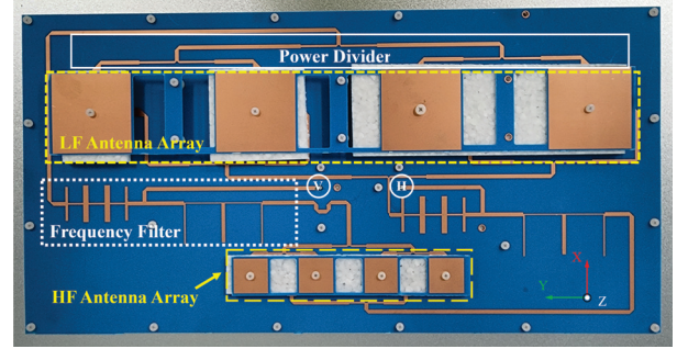
Fig. 8. Prototype of the dual-frequency dual-polarization antenna.
