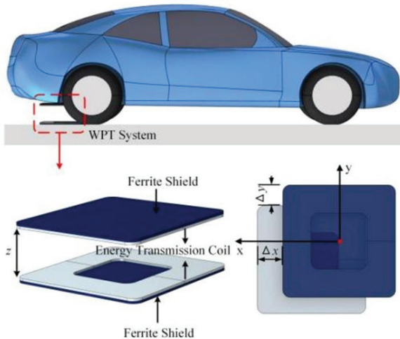
Fig. 1. Wireless charging of electric vehicles and the magnetic coupling mechanism.
