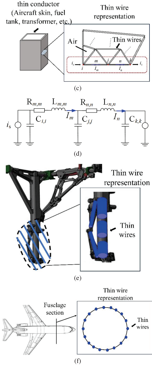
Fig. 1. Power PEEC of the thin-wire model. (a) Thin-line representation process of a high-voltage tower [27, 35], (b) thin-wire representation process of a grounding grid [35], (c) structures modeled as thin lines, (d) equivalent circuit diagram of some nodes and sticks, (e) thin-wire representation process of landing gear [30], and (f) thin-wire representation process of aircraft fuselage cross-section [25].
