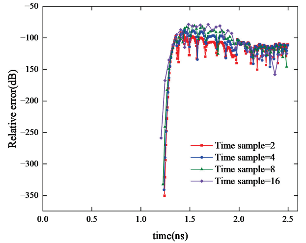
Fig. 7. Relative error of different time samples.
