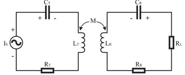
Fig. 2. EV-WPT system S-S compensation circuit.
