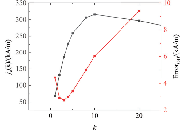
Fig. 7. Results of Error_{OD} and j_a(k) at different heights.
