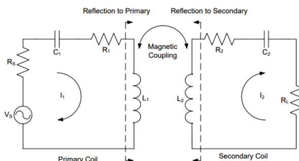
Fig. 3. Schematic diagram of inductive WPT [22].
