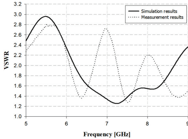
Fig. 7. VSWR results of the fabricated Vivaldi antenna.
