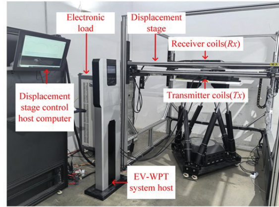
Fig. 9. Experimental setup.
