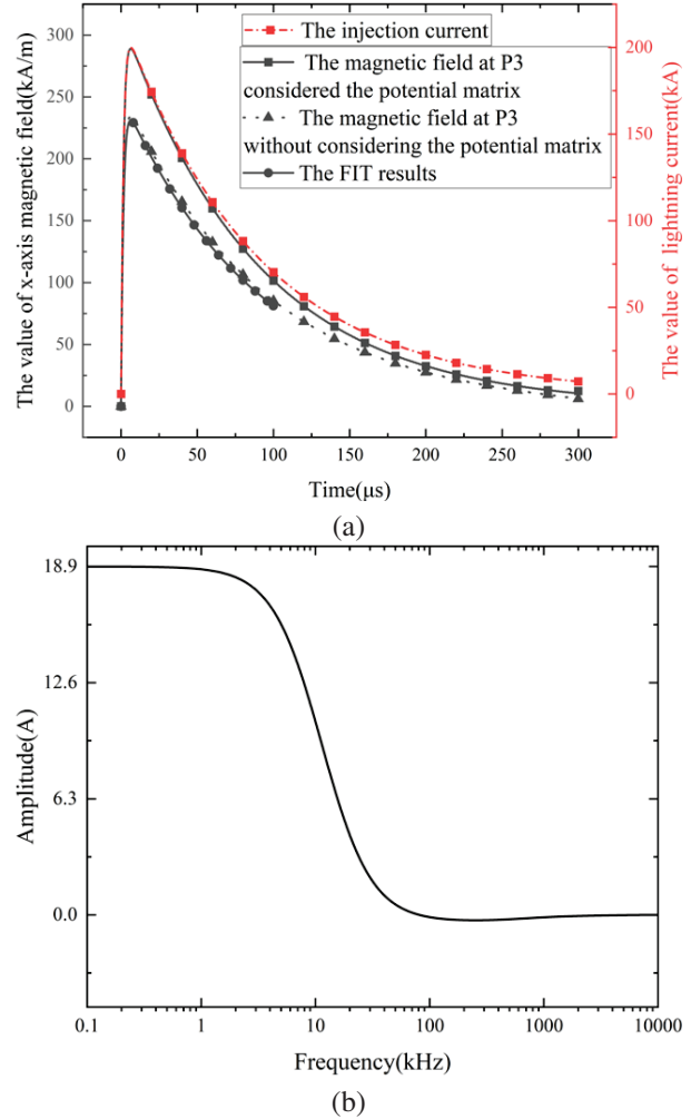
Fig. 5. Injected lightning current waveform and magnetic field waveform at the observation point. (a) Magnetic field waveform at position P3 and the injected current and (b) frequency component of lightning current component A.
