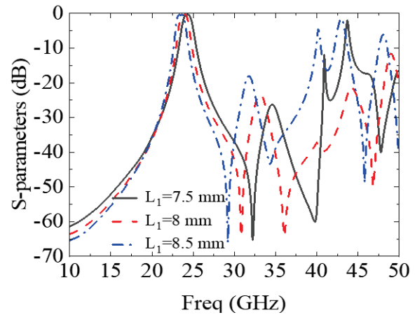
Fig. 5. Effects of different L_1 on the stopband of SIW filters.
