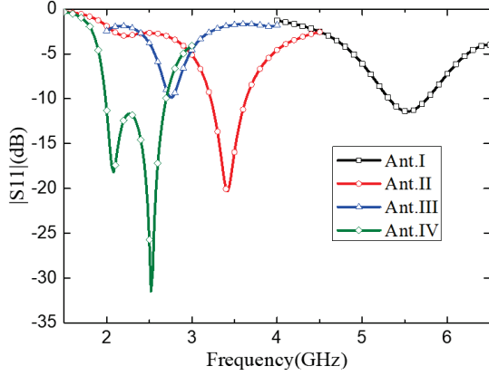
Fig. 3. Simulated |S_{11}| of the four evolution antennas.
