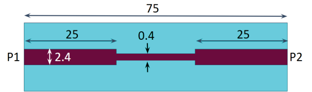
Fig. 15. A 50\Omega - 100\Omega - 50\Omega discontinuous microstrip line. All dimensions are in millimeters (mm).
