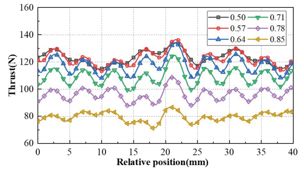
Fig. 18. Effect of core widths factor on thrust.
