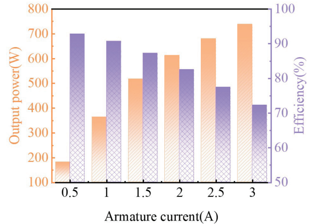
Fig. 29. Output power and efficiency of MFM-TFM with the variation of armature current.
