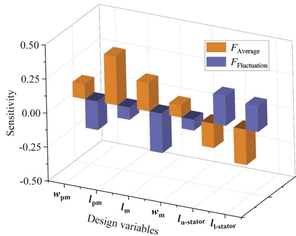
Fig. 24. Sensitivity analysis of optimization parameters to average thrust and thrust fluctuation.
