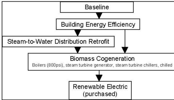
Figure 8. Cogeneration—Follow Electric Load
