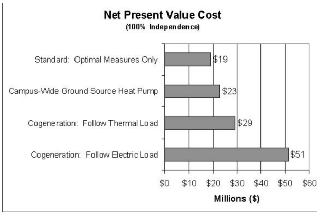
Figure 10. Life Cycle Cost Results
