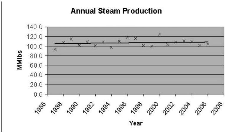
Figure 2. Annual Campus Steam Consumption
