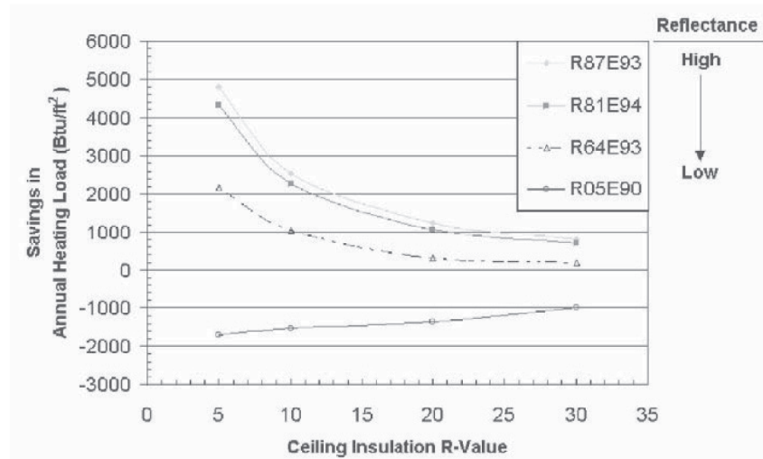
Figure 18. Annual heating load savings with offset-mounted PV
