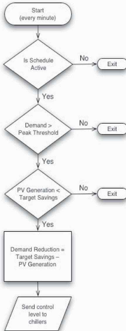
Figure 8. SLC control logic
