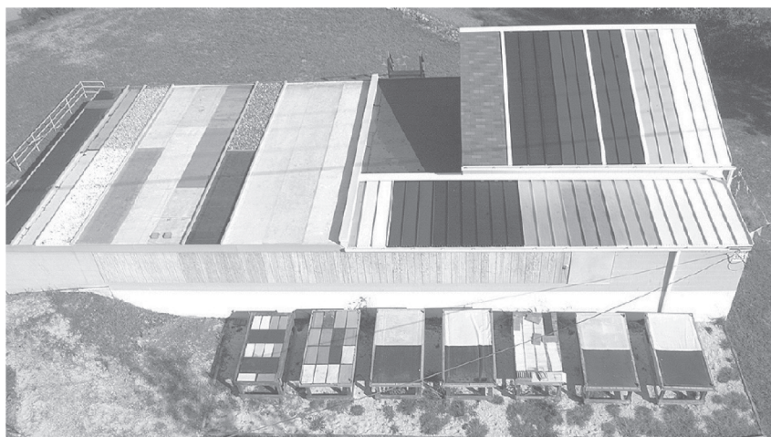
Figure 12. The Envelope Systems Research Apparatus used for testing painted and unpainted metal roofing
