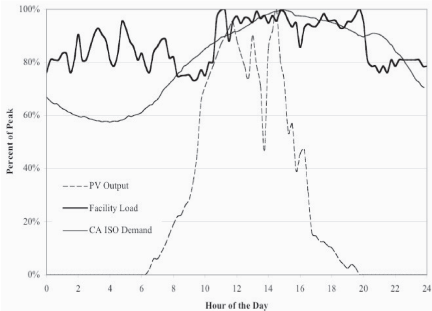
Figure 11. Relative PV performance on utility system peak day. Generation and load profiles for Marina PV array, Marina facility load, and CAISO system demand. Values have been normalized to the daily peak value for each data series. Data shown are for the day with the highest demand for the CAISO control area, July 10, 2002. Facility load is the end-use load, excluding the effect of PV generation.
