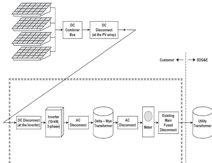
Figure 2. Layout of PV array, switchgear, and balance-of-system components
