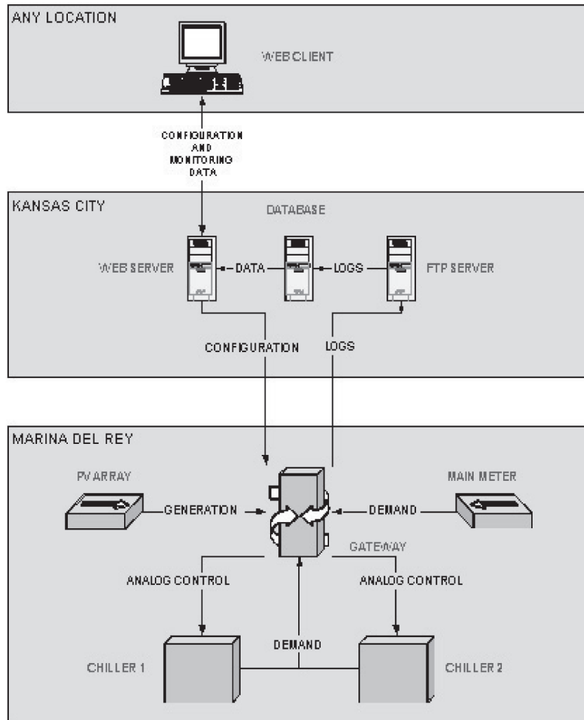
Figure 7. Marina Demand-Response System network configuration
