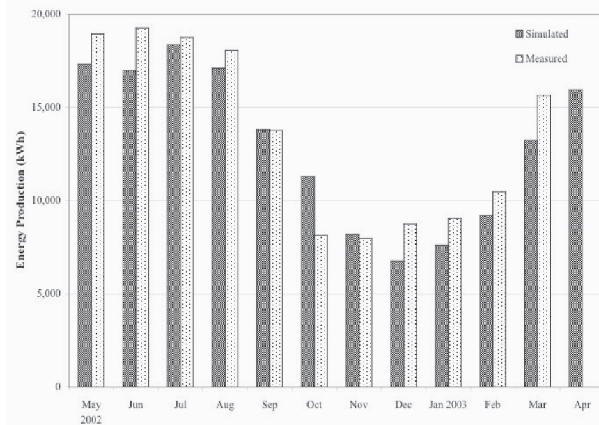
Figure 9. Comparison of estimated and measured energy production at USPS Marina Postal Processing Center. Measurements for April 2003 were not available yet. Actual production exceeded estimated amount by 6% for May–March. Actual production values for October–November may be under-represented because of measurement error (still under investigation).
