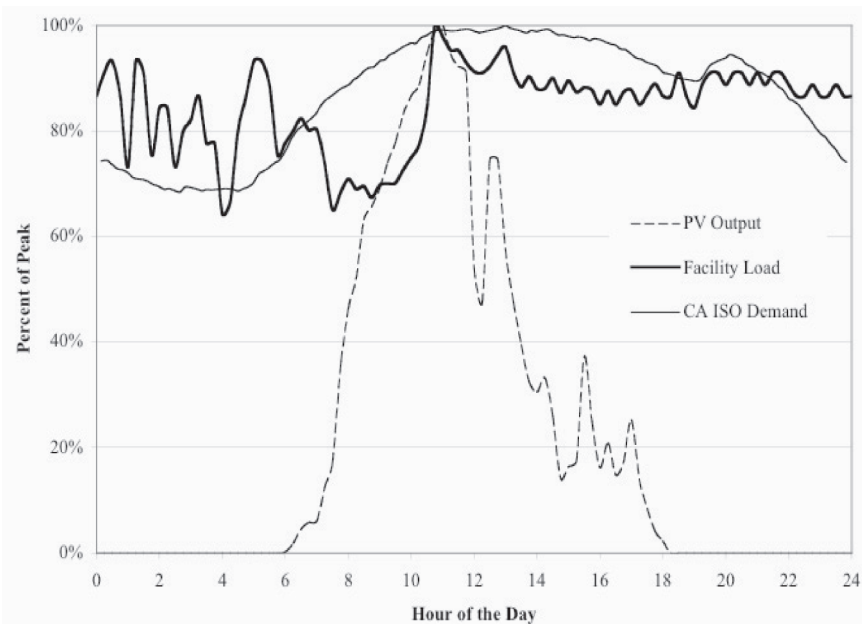
Figure 10. Relative PV performance on facility peak day. Generation and load profiles for Marina PV array, Marina facility load, and CA ISO system demand. Values have been normalized to the daily peak value for each data series. Data shown are for the day with the highest load for the facility, September 6, 2002. Facility load is the end-use load, excluding the effect of PV generation.
