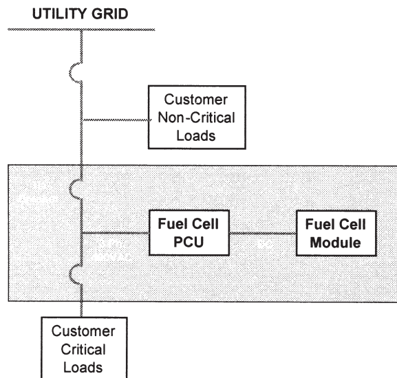
Figure 2. DFC300 typical configuration
