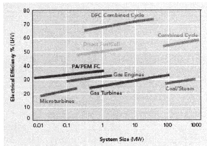
Figure 4. Efficiency comparison
