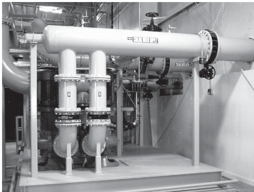
Figure 4. Skid-mounted equipment eases construction and replicability.
