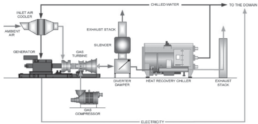
Figure 2. Integrated energy system includes natural gas turbine and heat recovery chiller.
