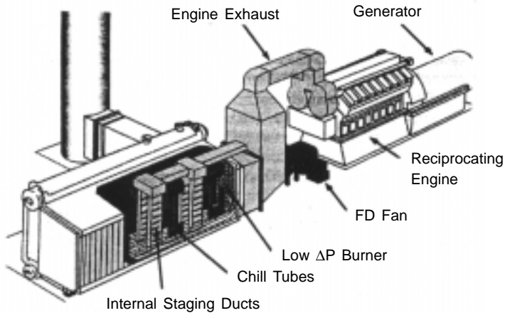
Figure 8. Integrated boiler burner*—advanced concept for midsized cogen or combined cycle plants. *Patent applied for.
