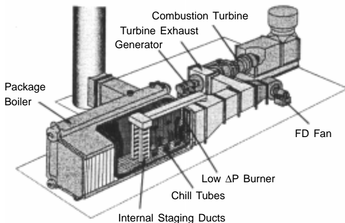
Figure 1. Integrated boiler burner*—advanced concept for midsized cogen or combined cycle plants. *Patent applied for.
