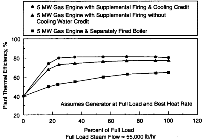
Figure 3. Plant efficiencies with various reciprocating engine configurations.
