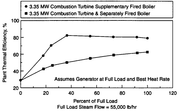
Figure 2. Plant efficiencies with various combustion turbine configurations.
