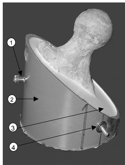
Figure 1. Fixation device of proximal femur: 1-screw 2-PVC sleeve 3-Epoxy resin F1 4-Treaded rod
