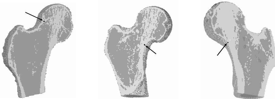
Figure 5. Location of the first element with reached failure limit
