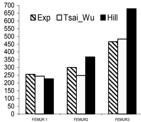
Figure 4. Experimental and numerical failure loads comparison (daN)
