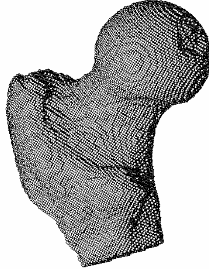
Figure 2. Voxel based mesh model of the first femur
