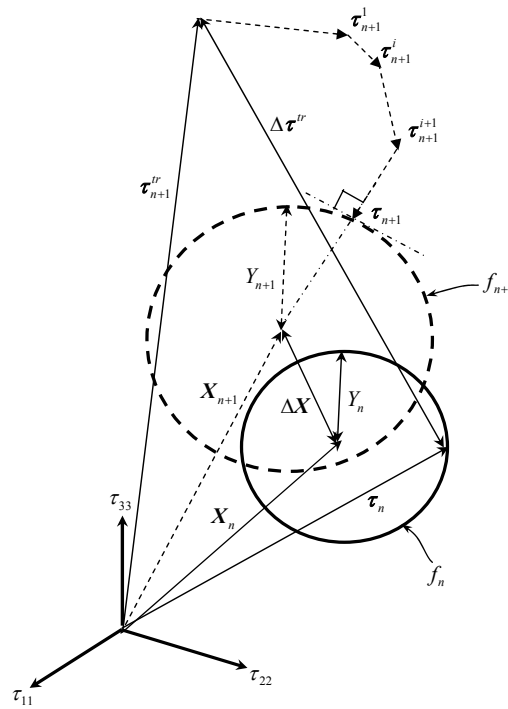
Figure 3. Conceptual representation of the Elastic predictor/ viscoplastic corrector algorithm
