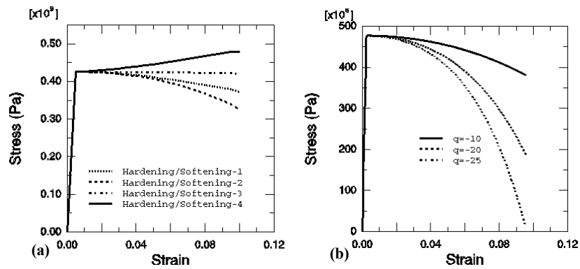
Figure 1. Behavior of the work-hardening-softening law Equation [8]. (a) 1 Q = -Q_M + (Q_o - Q_M) \exp(-qp) , 2 Q = Q_M + (Q_o - Q_M) \exp(qp) , 3 Q = 0 , 4 Q = Q_M + (Q_o - Q_M) \exp(-qp) , (b) Q = Q_M + (Q_o - Q_M) \exp(-qp)
