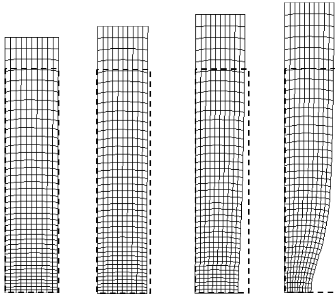
Figure 11. Deformation history for the 400 elements mesh corresponding to 2.5, 5, 7.5, and for 10 mm total elongation
