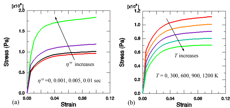
Figure 6. Uniaxial tension behavior obtained (a) for increasing relaxation times T = \eta^{vp} = 0, 0.001, 0.005, 0.01 \text{ sec} , and (b) for increasing temperature T = 0, 300, 600, 900, 1200 \text{ K}
