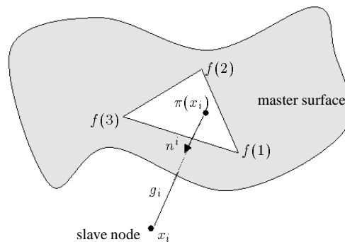
Figure 4. Master-slave pair
