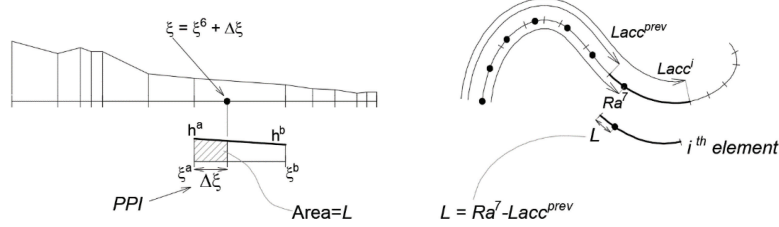
Figure 14 Example for the calculation of the seventh vertex.
