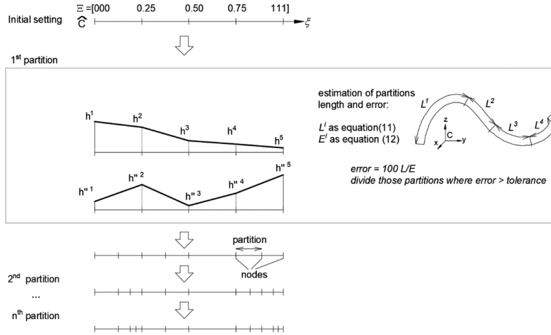
Figure 12 dC-mesh division process with first step detailed.
