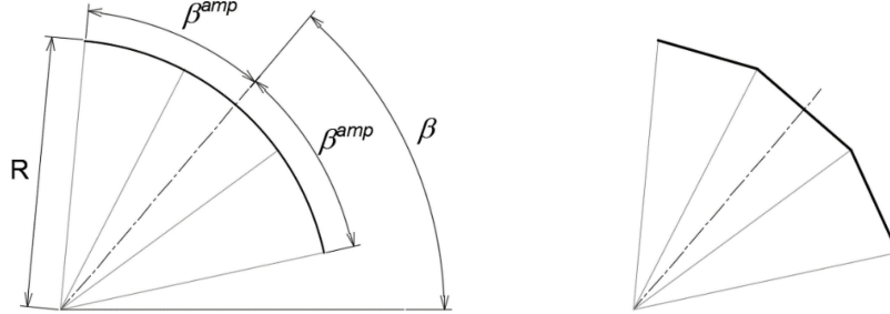
Figure 20 Definition of arc and discretization into three lines.
