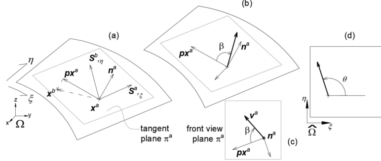
Figure 23 Calculation of angle \theta correspondent to the \beta angle. Computation of the \pi^a plane and projected vector px^a (a); local base B^a (b); vector with \beta angle v^a (c); corresponding angle \theta in the parameter space (d).
