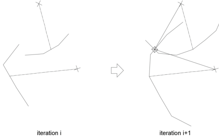
Figure 26 AIP case C in the parameter space.
