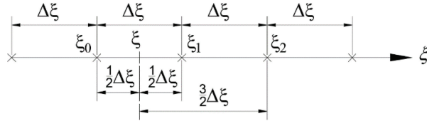
Figure B.3 Location of representative coordinate \xi .
