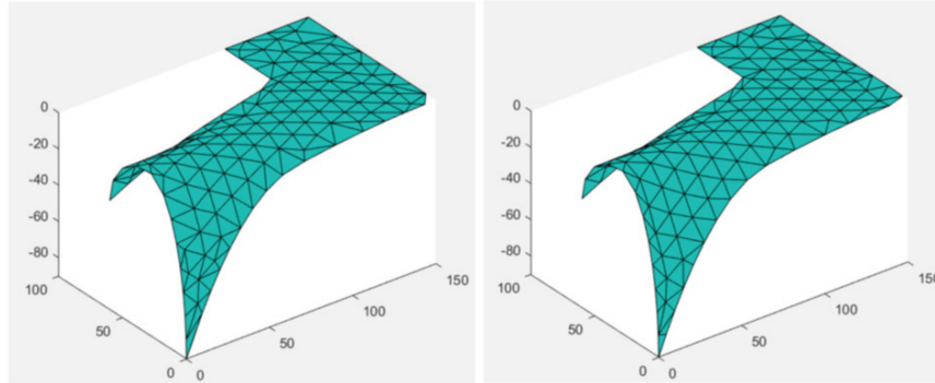
Figure 40 Triangulation for tolerances of 4.0 % (left) and 0.25% (right).
