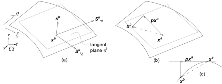
Figure 21 Tangent plane obtained by cross product of the derivatives to the surface (a). Projected vector px^a onto the \pi^a plane (b). Front view of the projection's procedure at the right-bottom (c).
