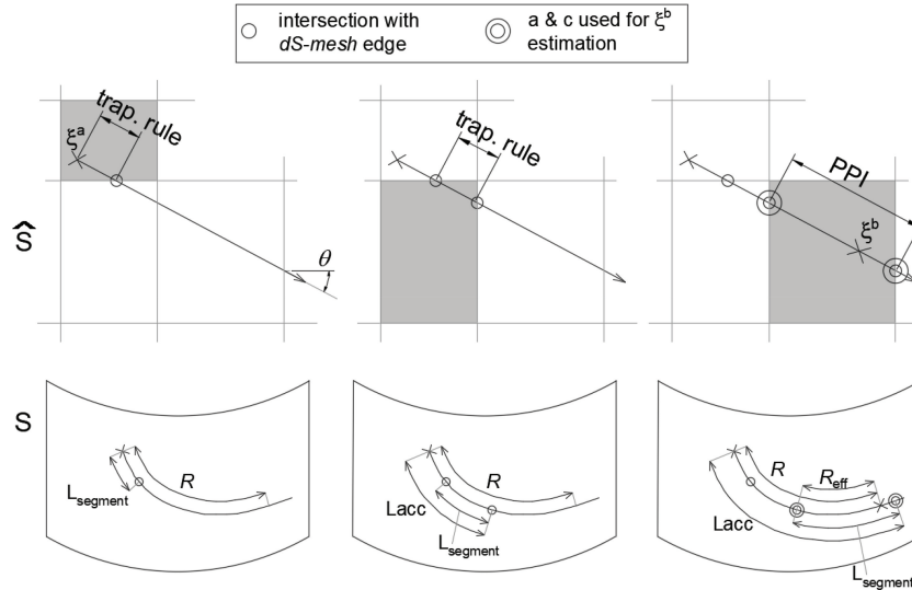
Figure 18 Estimation of different path increments to achieve the physical target distance R . Above represents the parameter space, with grey hatching the partition of dS-mesh involved. Below it is detailed the path in the physical space.
