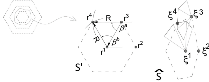
Figure 27 Fourth vertex computation.
