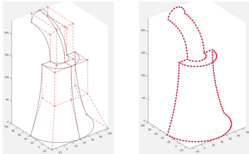
Figure 41 Left: surfaces for triangulation. Right: edge vertexes resultant from the QIT algorithm.
