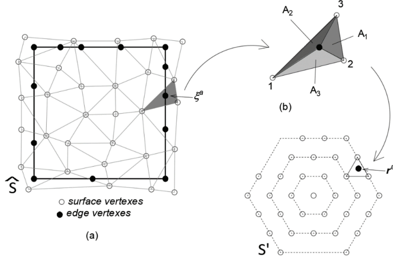
Figure 30 Triangulation of all vertices in the parameter space (a) and calculation of the pattern coordinates of the edge vertex a (b).
