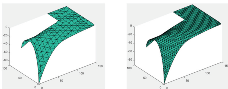
Figure 34 Resultant QIT triangulation. Left: R = 12 . Right: R = 5 .
