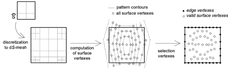
Figure 9 Computation of surface vertexes .
