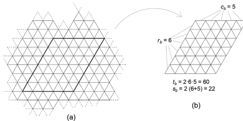
Figure C.1 Ideal isotropic triangulation (a) and extraction of 6 \times 5 BIT (b).
