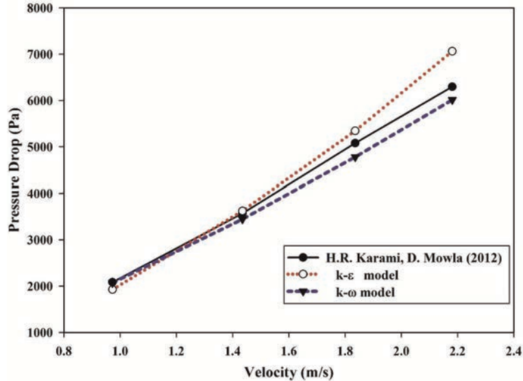
Figure 22 Comparison between k - \epsilon and k - \omega models pressure drop and the experiment pressure drop for H.R. Karami, D. Mowla. Ref. [16].
