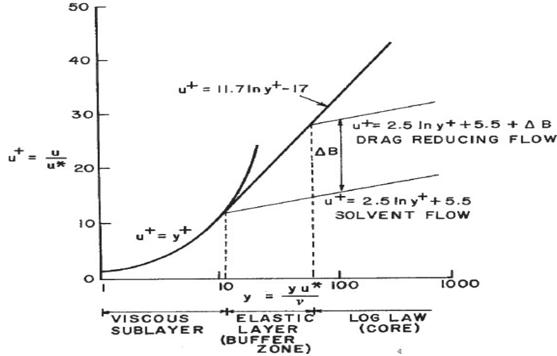
Figure 2 Velocity distribution in the boundary layer for polymer drag reduction based on typical velocity profile model for turbulent flow (from Sillin et al. Ref. 30).
