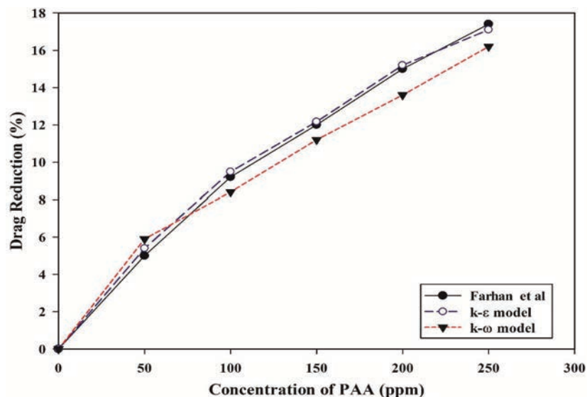
Figure 7 Simulated Drag reduction percentage for crude oil flow rate with different PAA concentration compared with experimental data for Farhan et al. Ref. [14].
