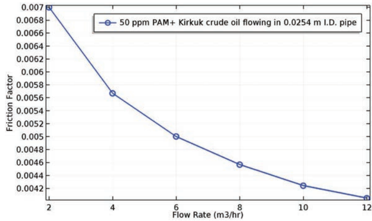
Figure 16 Simulated k - \omega model friction factor for crude oil with 50 ppm PAM ( \Delta B = 0.65 ) flowing in 0.0254 m diameter, at different flow rates for Ali A. Abdul-Hadi (2013, Ref. [4]).
