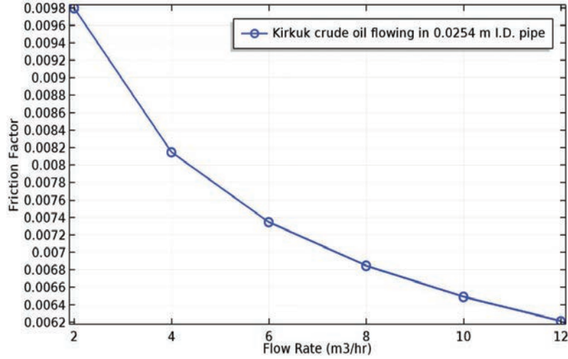
Figure 15 Simulated k - \epsilon model friction factor for crude oil ( \Delta B = 0 ) flowing in 0.0254 m diameter, at different flow rates for Ali A. Abdul-Hadi (2013, Ref. [4]).
