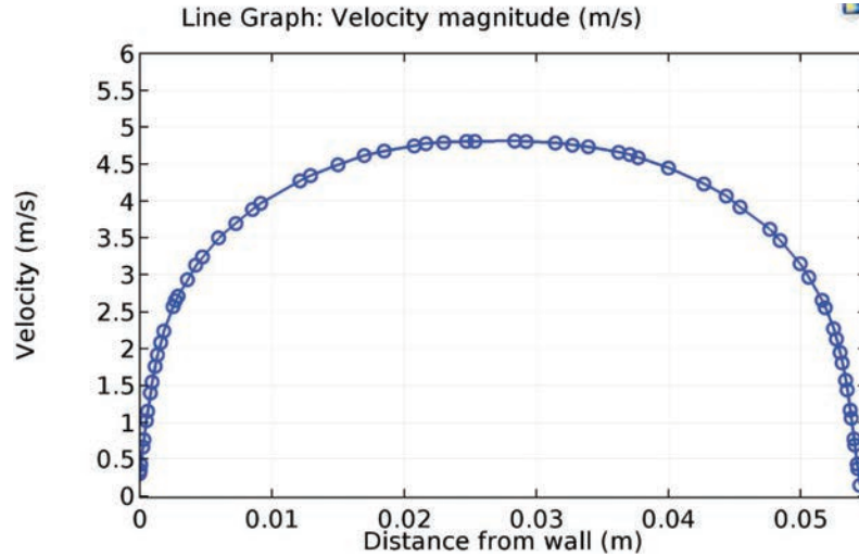
Figure 19 Simulated k - \omega velocity profile at the entrance length for Farhan et al. Ref. [14].
