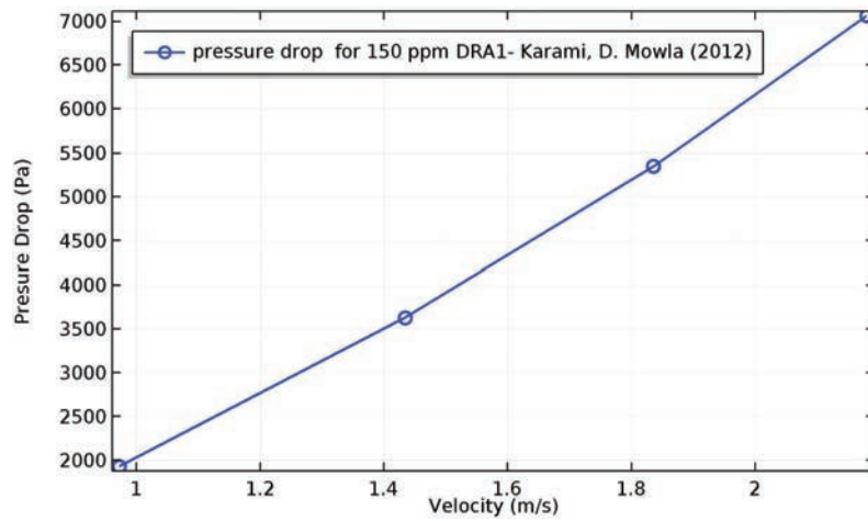
Figure 21 Simulated pressure drop versus velocity for crude oil with 150 ppm DRA1 for H.R. Karami, D. Mowla. Ref. [16].
