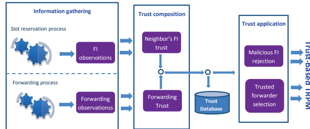
Figure 3 General Architecture of the proposed Trust-aware cross-layer routing protocol.
