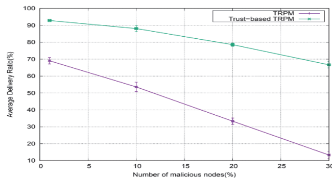
Figure 6 Black Hole attacks: Average delivery ratio vs Number of malicious nodes in the case of 43 vehicles.
