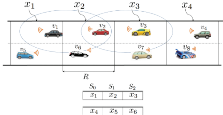
Figure 1 TDMA slots scheduling principle.
