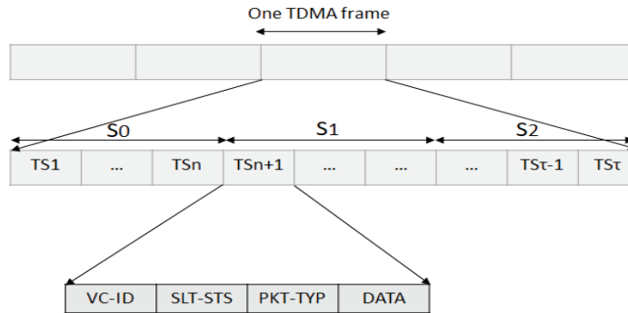
Figure 2 Frame Information (FI) structure.
