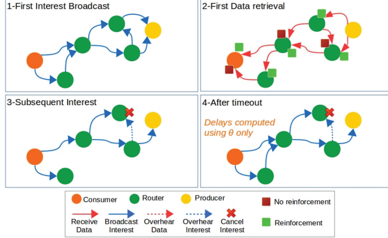
Figure 7 Common forwarding situations with R-LF.
