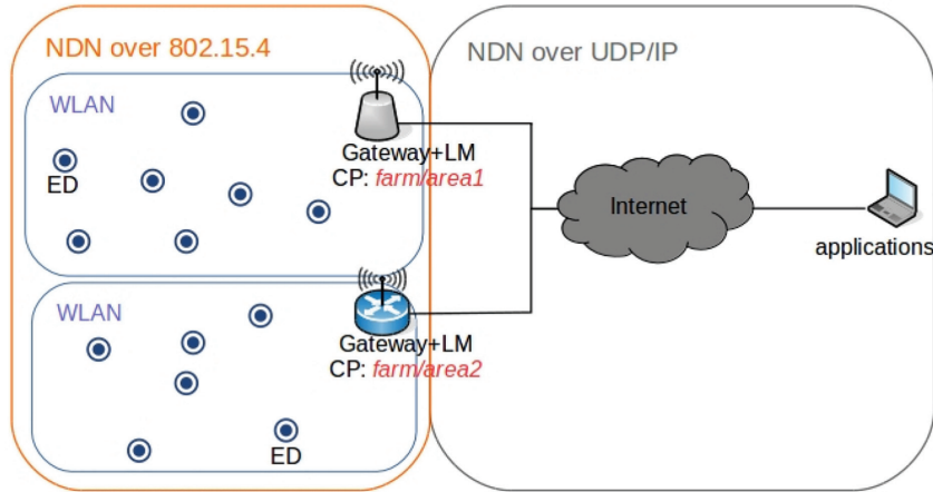
Figure 5 NDN-802.15.4 architecture.
