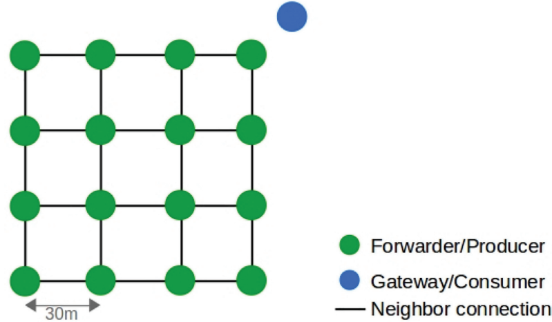
Figure 14 Simulated topology.
