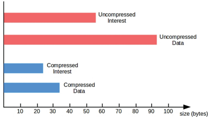
Figure 13 Compression improvement.
