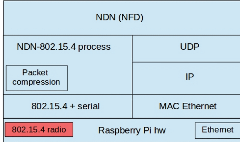
Figure 9 Architecture of the gateway.
