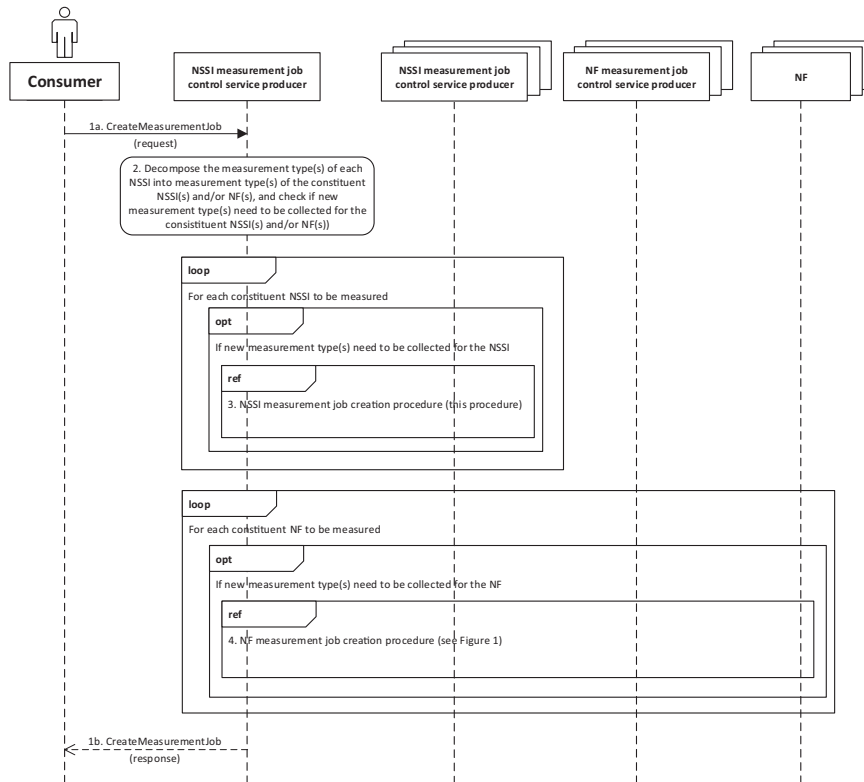
Figure 2 Procedure for NSSI measurement job creation.
