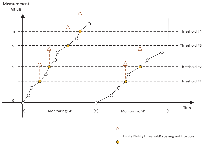
Figure 6 Threshold crossing notifications triggering for cumulative counters.
