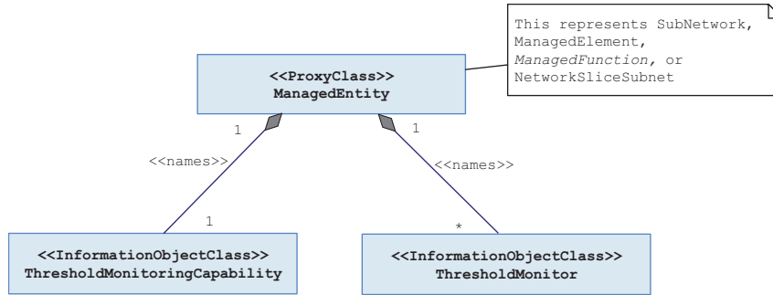
Figure 5 Threshold monitor models.
