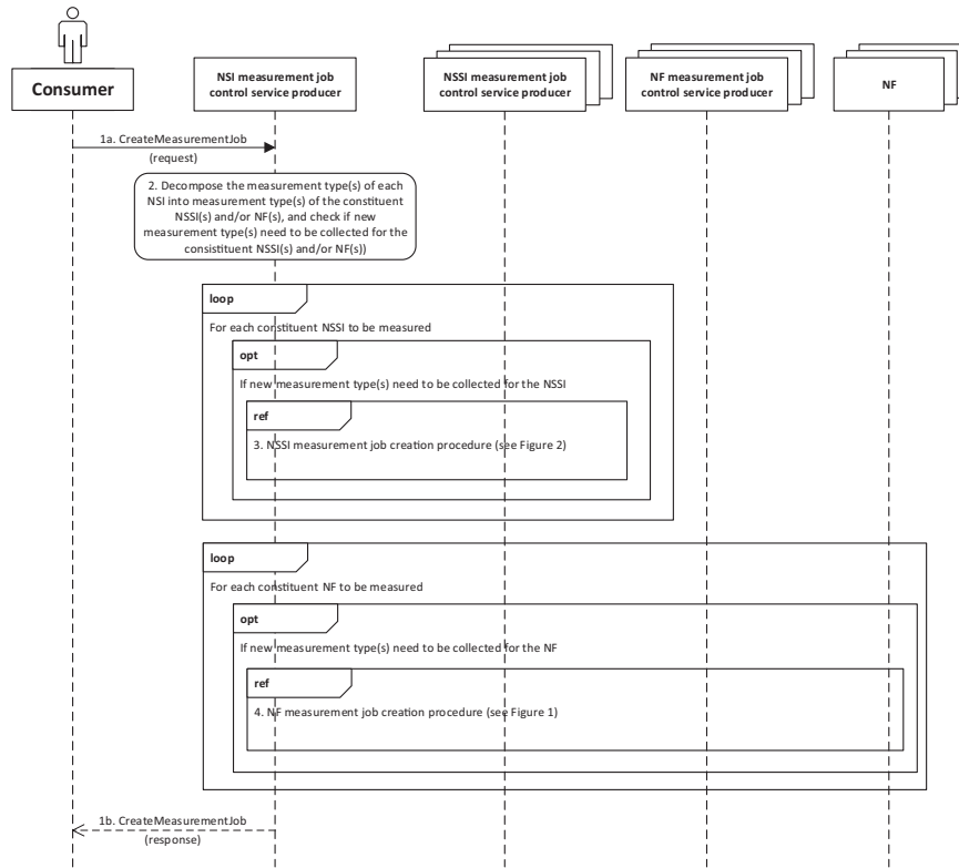
Figure 3 Procedure for NSI measurement job creation.
