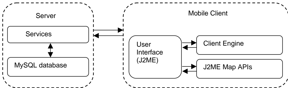
Figure 1. The architecture of the MobiTOP system.
