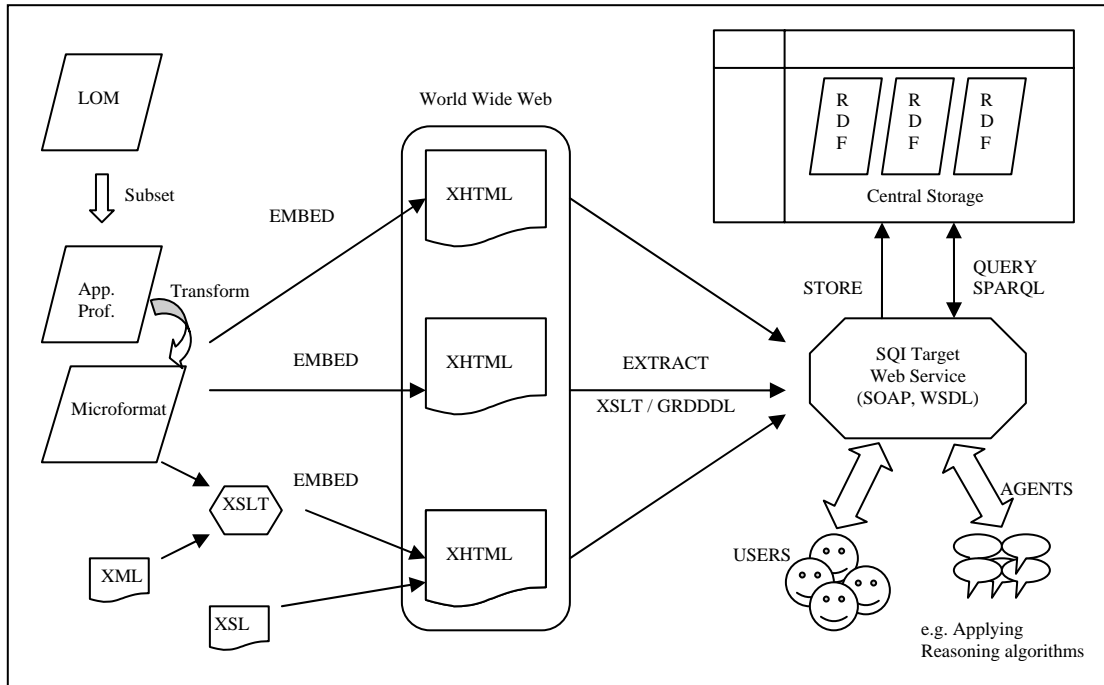
Figure 12. Partially implemented extended framework.
