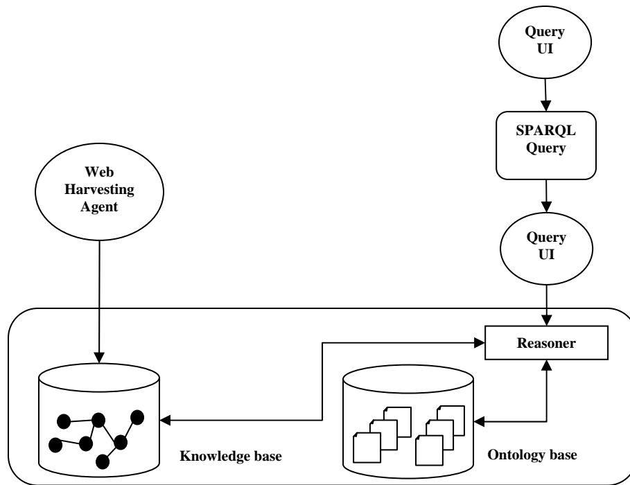
Figure 11. The extended framework demonstrating proposed web harvesting procedure with ontology support.
