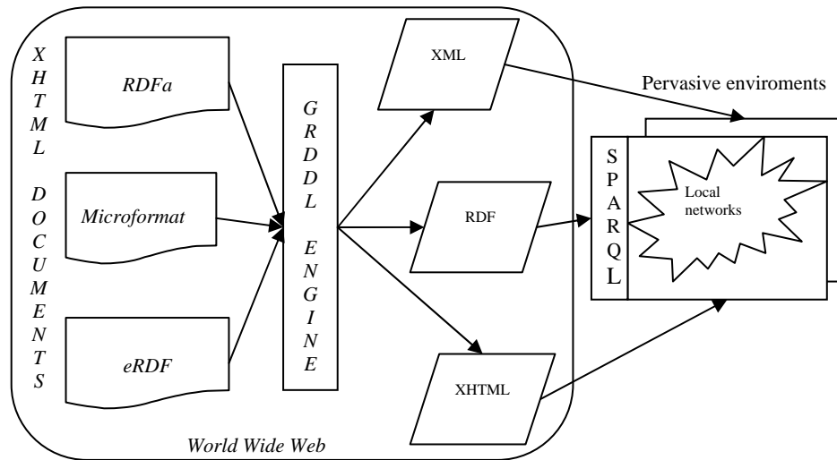
Figure 6. A simple web harvesting framework.
