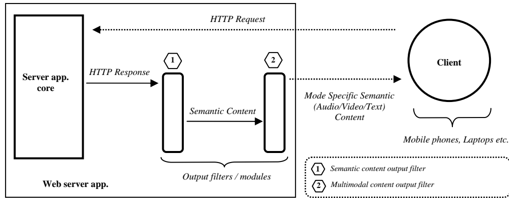
Figure 15. (1) Semantic content output filter, and (2) multimodal content output filter.
