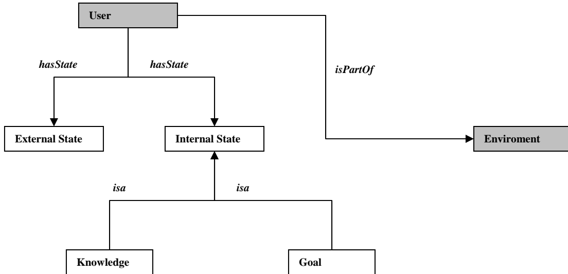
Figure 2. First part of the proposed upper context conceptualization; external state and internal state concepts are shown as a part of user concept where user concept is part of the environment [16].
