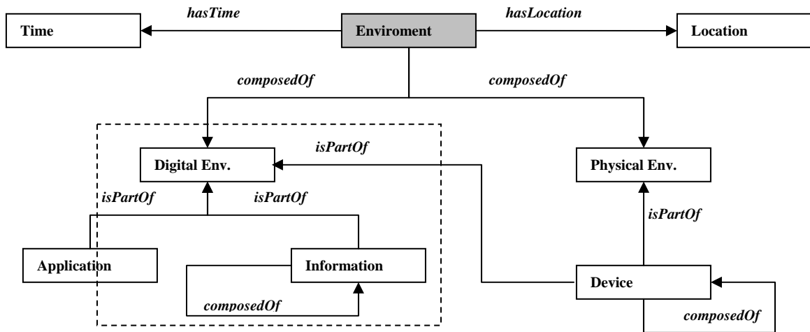
Figure 3. Second part of proposed upper context conceptualization; environment concept is composed of digital environment and physical environment concepts [16].
