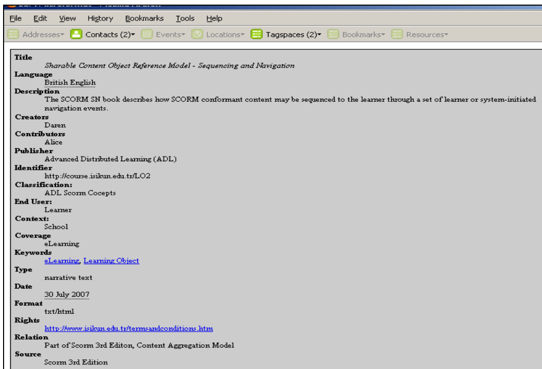
Figure 13. Extracted metadata of an exemplary learning object encoded with our Microformat.
