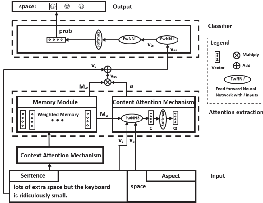
Figure 1 CABASC framework.
