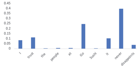
Figure 6 Content attention.
