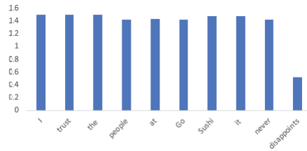
Figure 7 Context attention.
