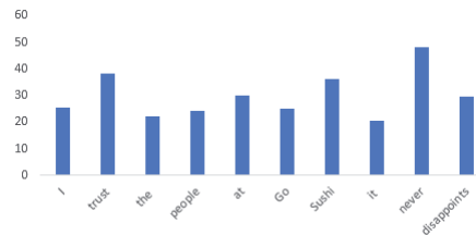
Figure 8 Content attention.
