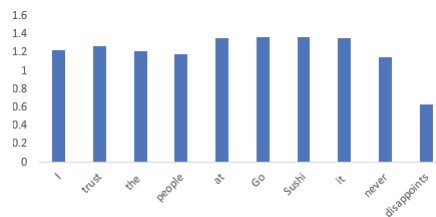
Figure 9 Context attention.
